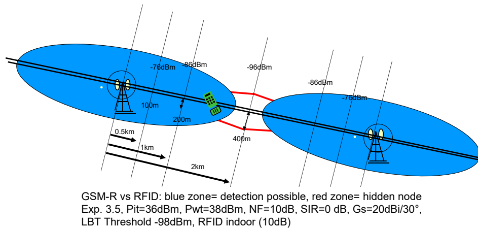
Figure 67: Hidden nodes (red areas) and detection areas (blue), RFID indoor
