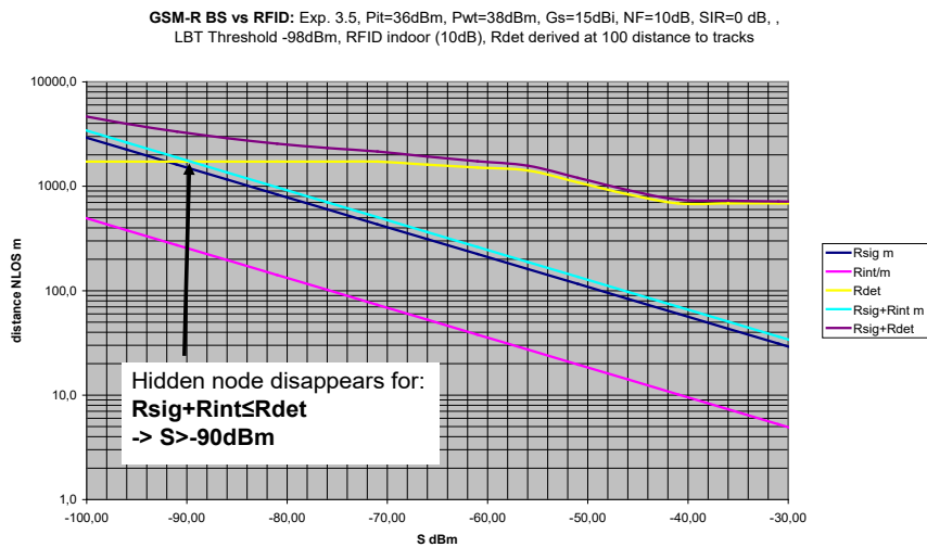
Figure 65: Calculated area sizes for indoor RFID case
