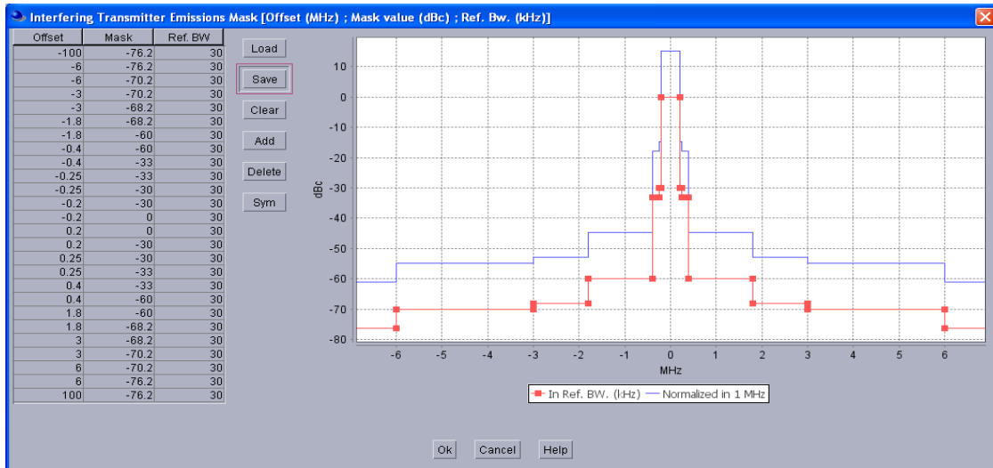
Figure 17: Unwanted emissions mask of GSM-R MS (based on GSM MS specs)
