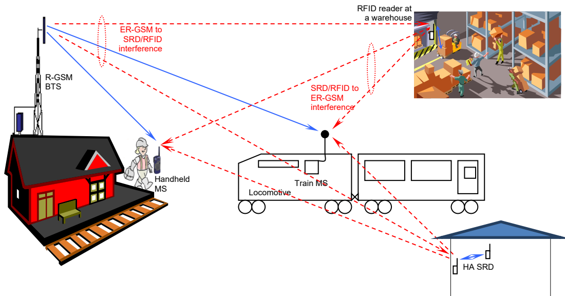
Figure 54: In-band SRD/RFID vs. ER-GSM co-existence: wanted and interfering paths in 918-921 MHz
