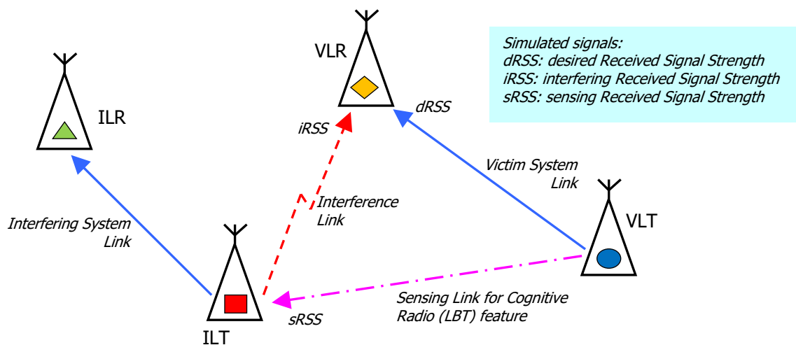
Figure 39: Modernised representation of SEAMCAT scenario elements
