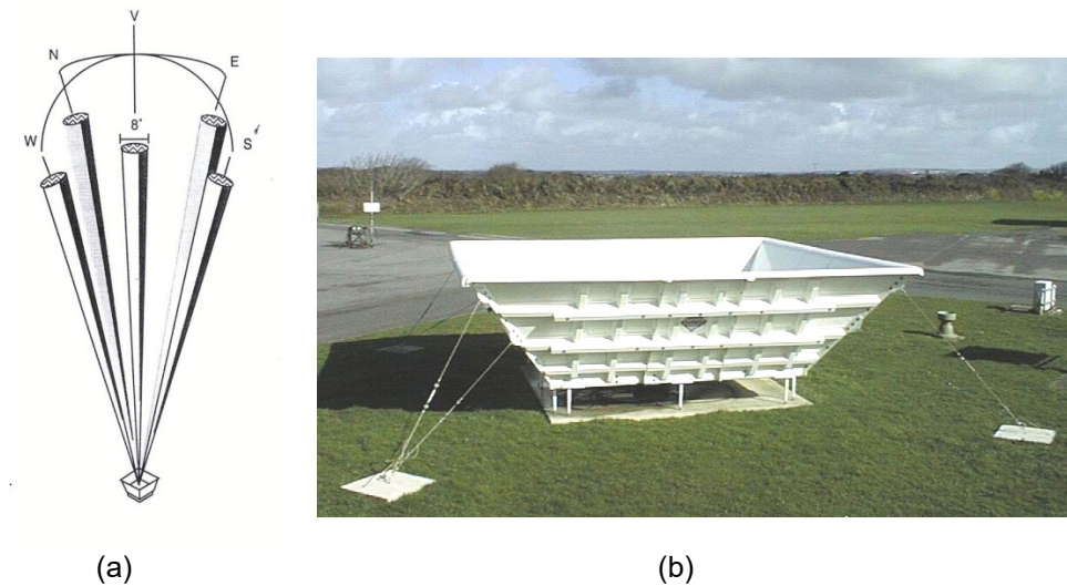
Figure 27: Wind Profiler Radar antenna beams (a) and installation within screened enclosure (b)
