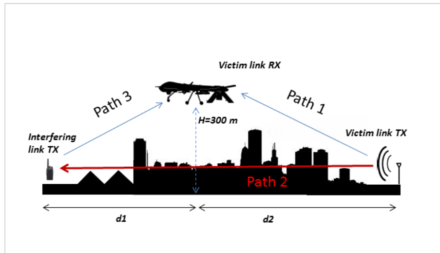
Figure 44: Considered DAA sensing configuration for UAS scenarios
