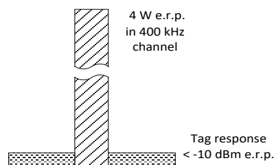
Figure 28: The RFID transmissions arrangement in dense interrogator mode
