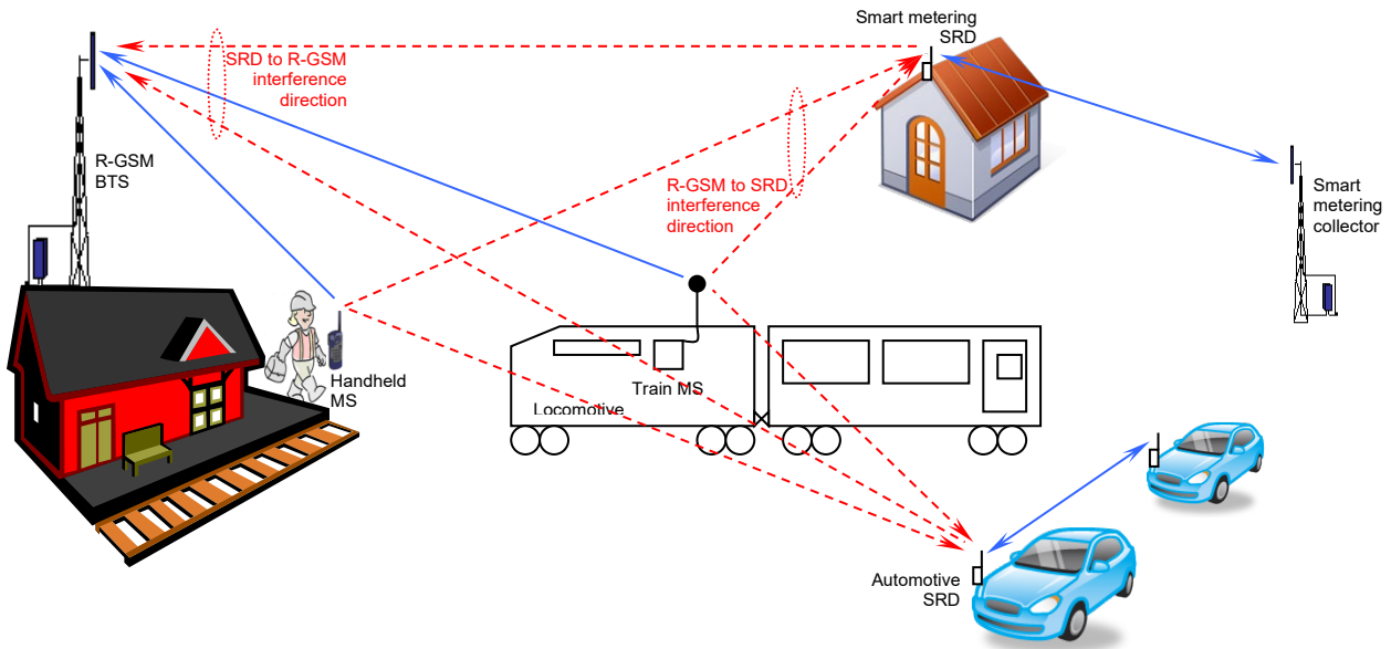
Figure 7: In-band SRD vs. ER-GSM co-existence: wanted and interfering paths in 873-876 MHz
