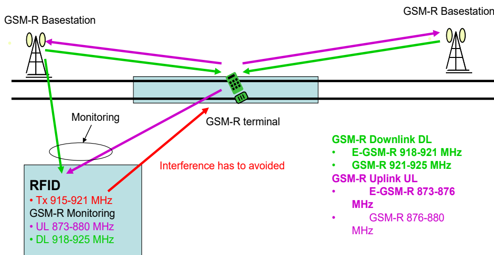
Figure 61: Illustration of concept of spectrum sensing by RFID
