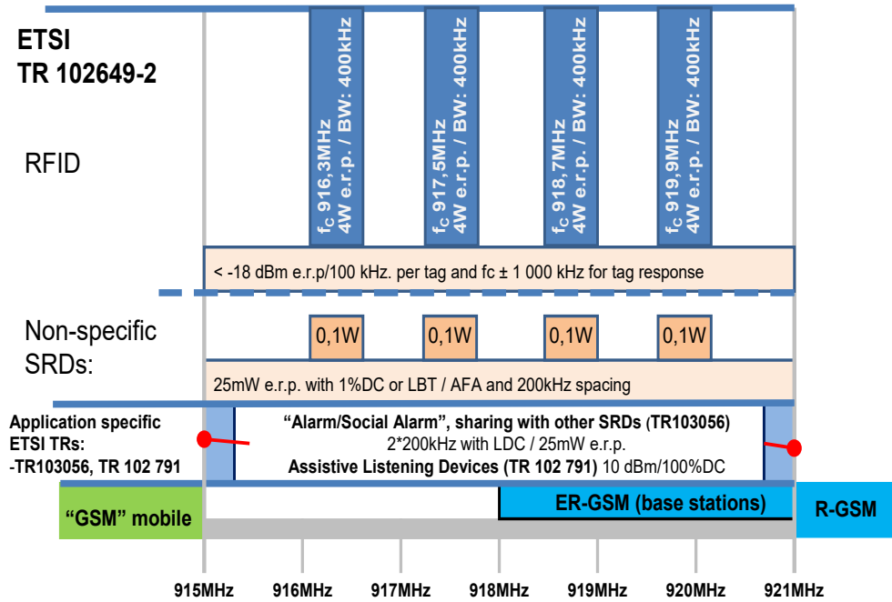
Figure 38: The summary of the updated SRdocs outlining SRD/RFID requirements in the band 915-921 MHz
