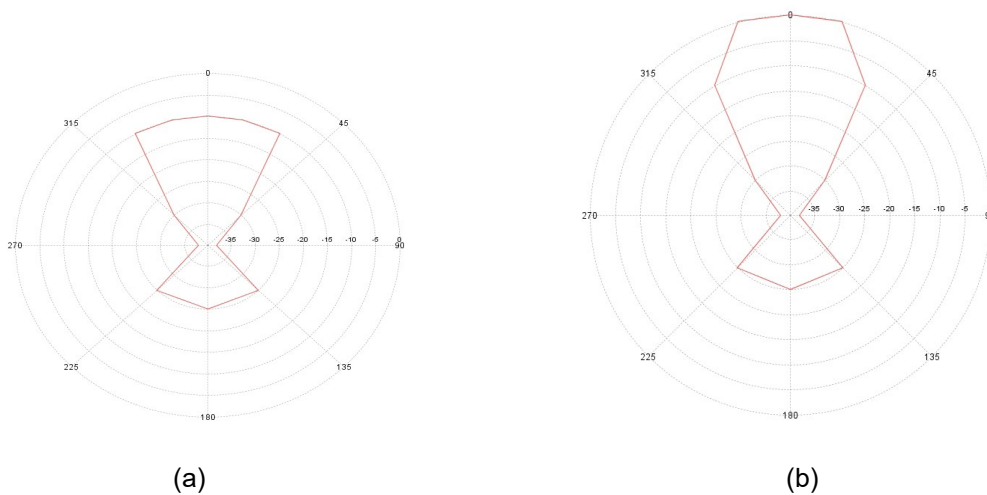
Figure 29: Radiation pattern of RFID interrogator antenna Type 1 (a) and Type 2 (b)
