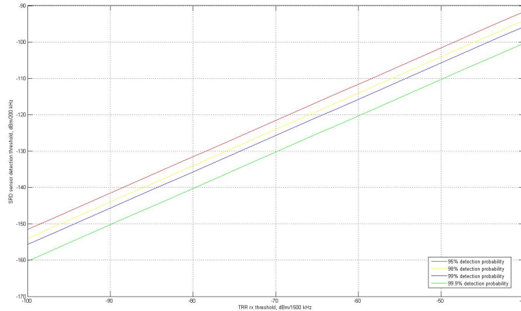
Figure 43: Required DAA sensing threshold as a function of mean level of TRR wanted signal
