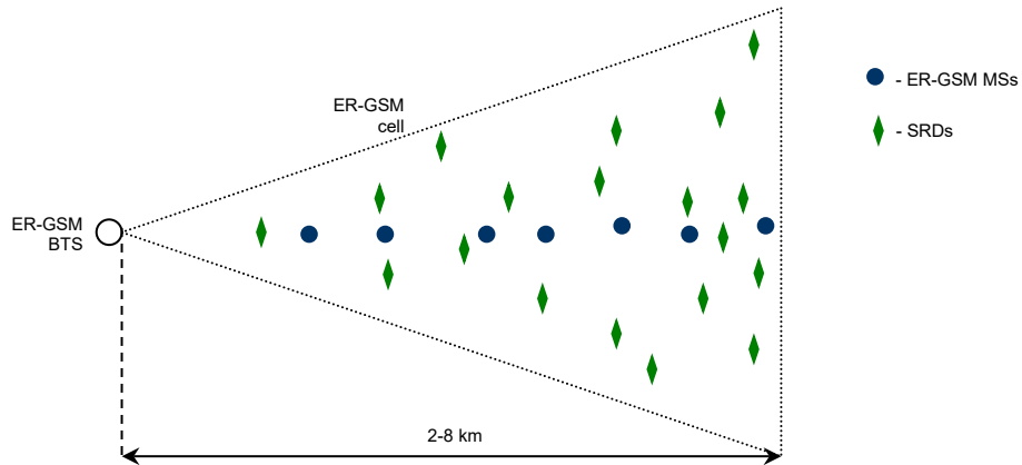
Figure 8: Geographic representation of SRD vs. ER-GSM co-existence scenario in SEAMCAT
