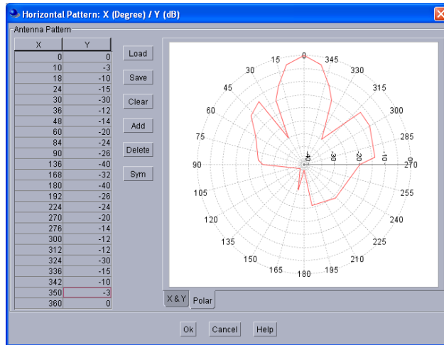
Figure 23: Radiation pattern of TRR antenna [18]
