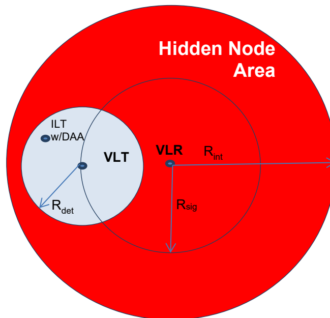
Figure 40: Illustration of DAA sensing deficiency zone (Hidden Node), adapted from ECC Report 181 [31]
