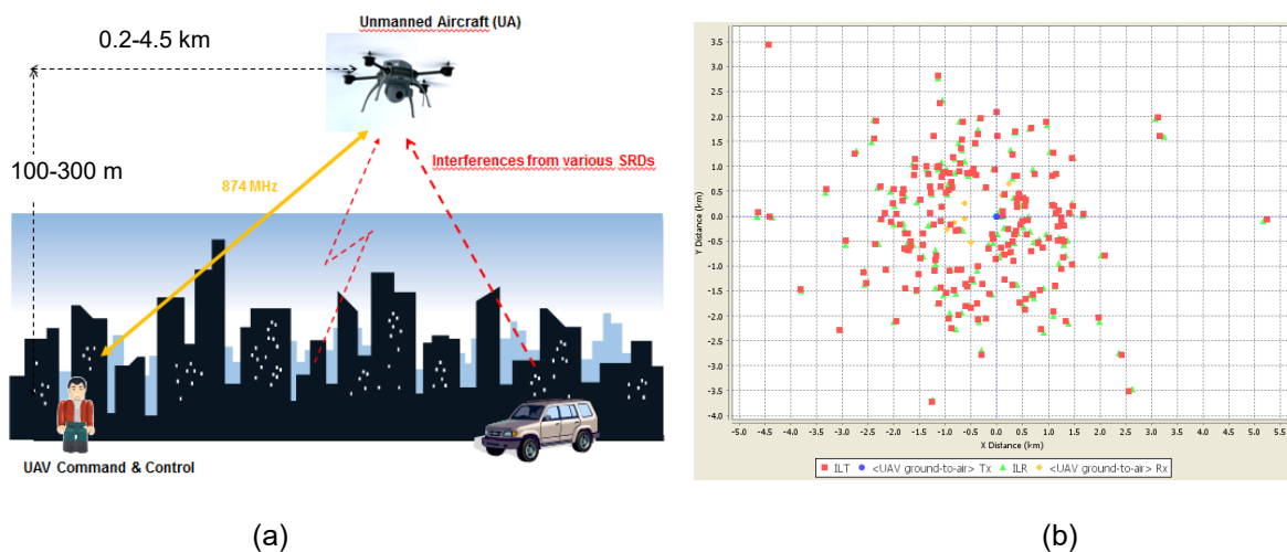
Figure 4: Scenario of SRD vs. UAS co-existence in 870-876 MHz: (a) – general vision in urban environment, (b) – snapshot view in SEAMCAT with 10 active interferers
