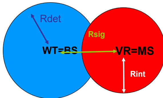
Figure 64: Illustration of the analysed hidden node scenario
