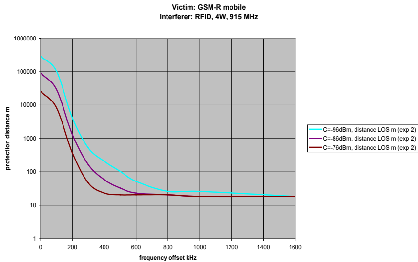
Figure 56: Protection distance between RFID interrogator and ER-GSM mobile under LOS conditions
