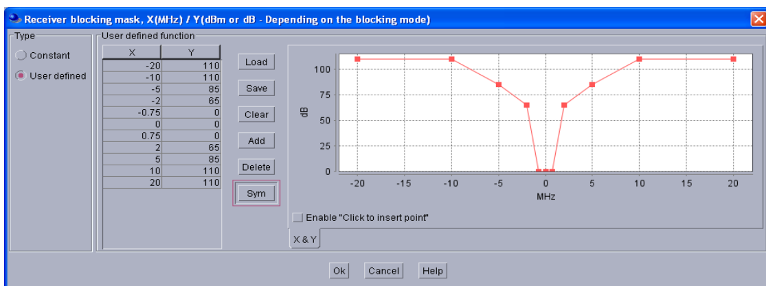
Figure 25: Receiver blocking function of TRR (ref. STANAG-4212 [18])
