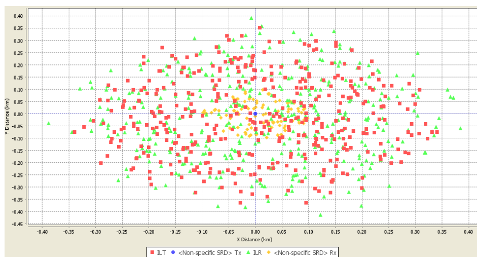
Figure 12: Example of SEAMCAT simulation window: Intra-SRD co-existence scenario
