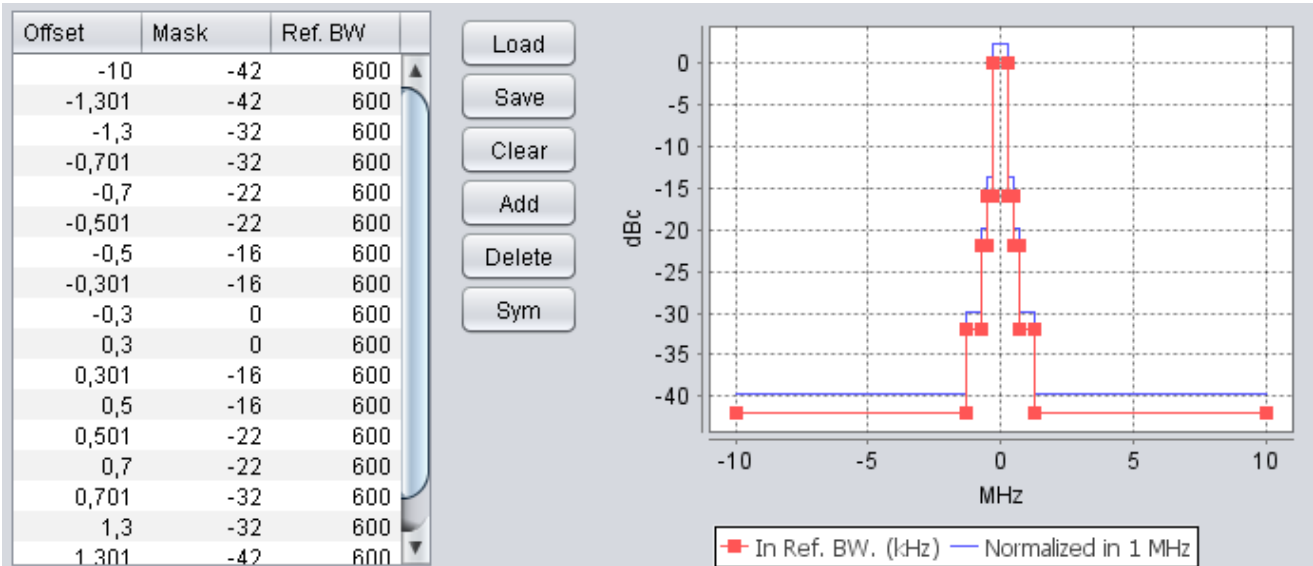
Figure 33: Non-specific Type A
