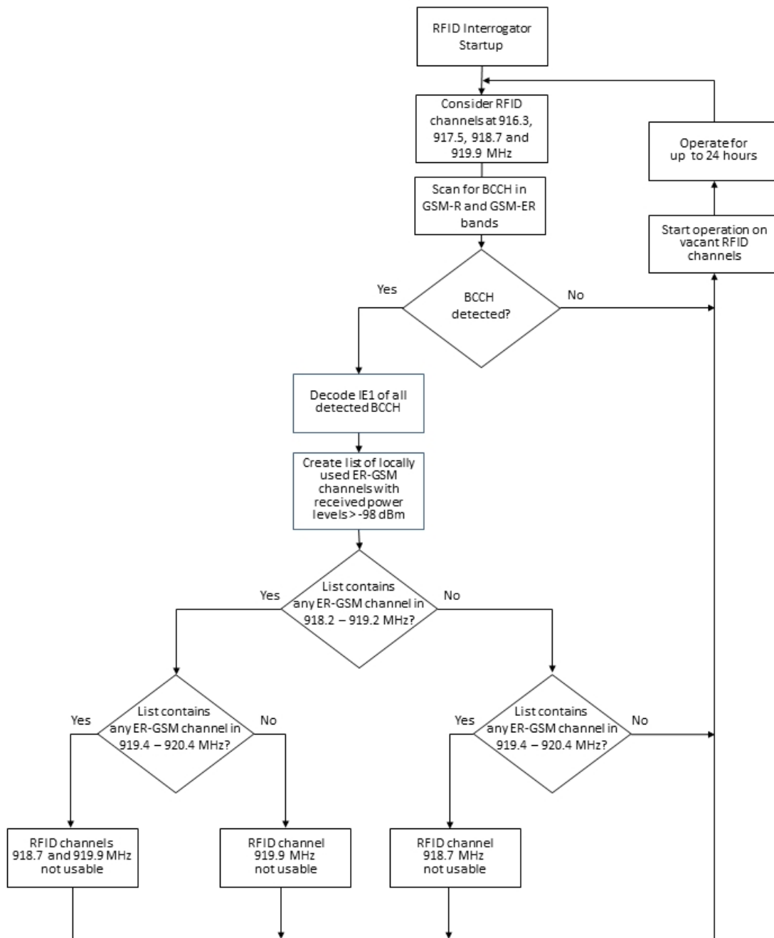
Figure 62: GSM-R Downlink detection for ER-GSM band and RFID DAA process
