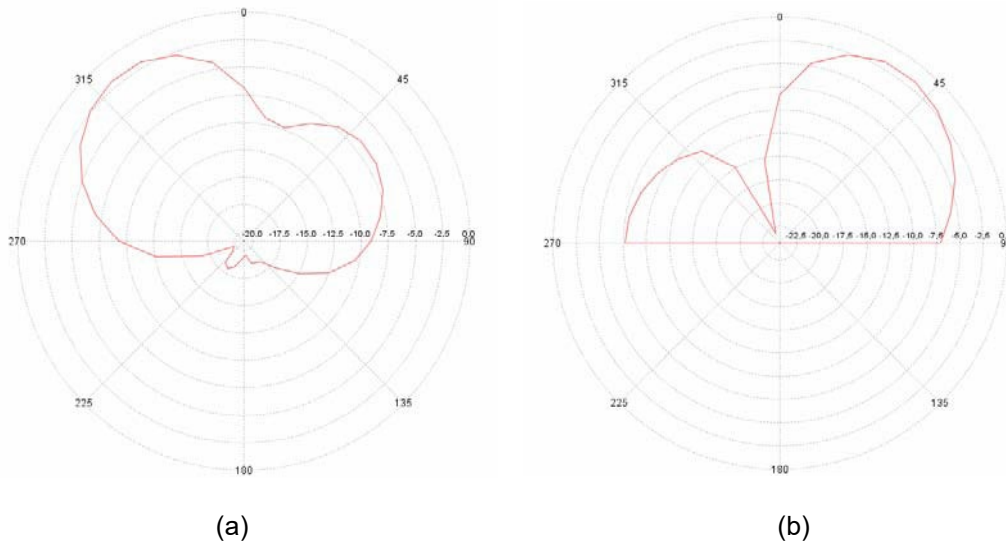
Figure 30: Radiation patterns of RFID antenna Type 3: horizontal (a) and vertical (b) planes
