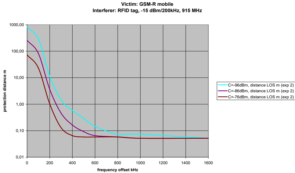
Figure 58: Protection distance between RFID tags and ER-GSM mobile under LOS conditions
