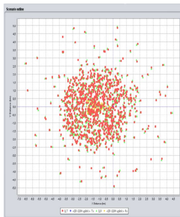
Figure 11: Outline of SEAMCAT simulations reported in this section
