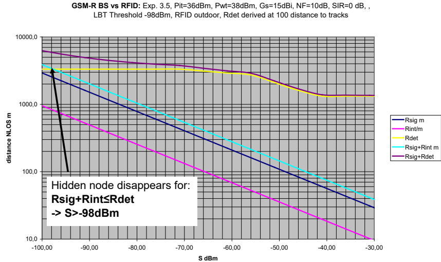
Figure 66: Calculated area sizes for outdoor RFID case
