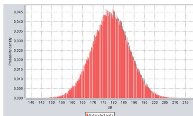
Figure 45: Simulated path loss on DAA sensing path in UAS scenarios
