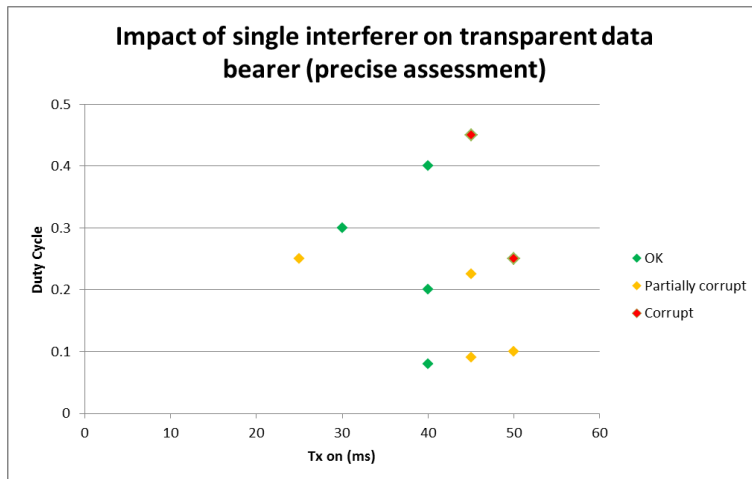
Figure 49: Impact of a single interferer on a transparent data bearer (precise assessment)
