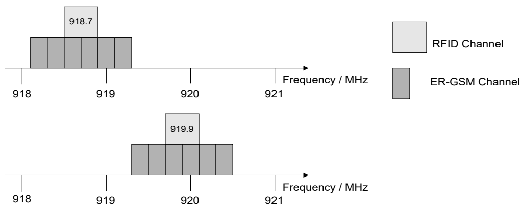
Figure 63: Illustration of interference between ER-GSM and RFID channels
