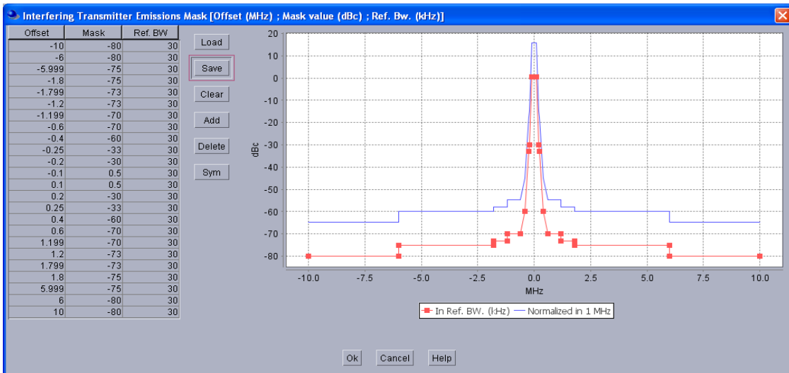
Figure 18: Unwanted emissions mask of GSM-R BTS [22]
