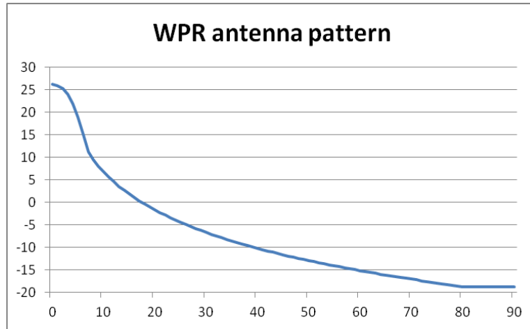
Figure 26: Antenna pattern of Wind Profiler Radar at 915 MHz
