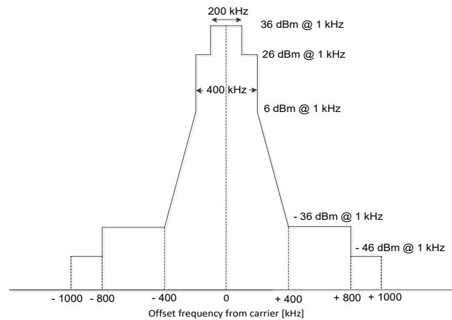
Figure 31: Spectrum emissions mask of RFID interrogator’s transmitter
