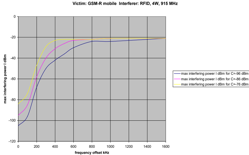
Figure 55: Main results of ETSI TR 101 537: max acceptable interference power at ER-GSM receiver
