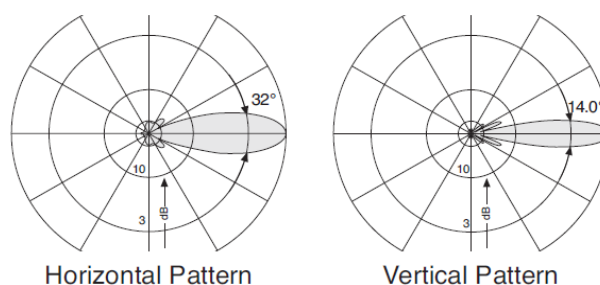
Figure 16: Radiation pattern of directional GSM-R BTS antenna (ref. Kathrein Type 80010642)
