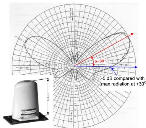
Figure 15: Example of train-mounted GSM-R MS antenna and its vertical radiation pattern [23]
