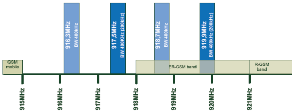
Figure 3: Tentative band plan for 915-921 MHz, based on amended TR 102 649-2 [2] proposal
