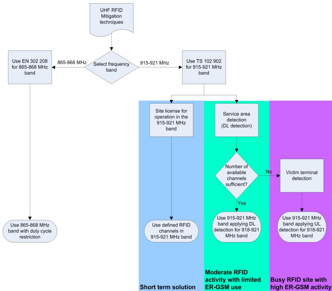
Figure 60: Overall coexistence strategy between ER-GSM and RFID
