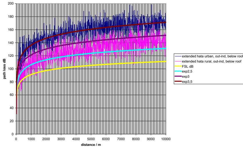
Figure 10: Choosing propagation exponents to represent Extended Hata rural and urban modes
