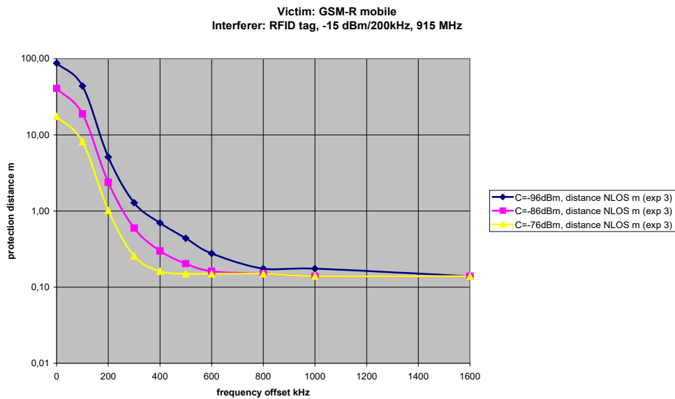
Figure 59: Protection distance between RFID tags and ER-GSM mobile under NLOS conditions
