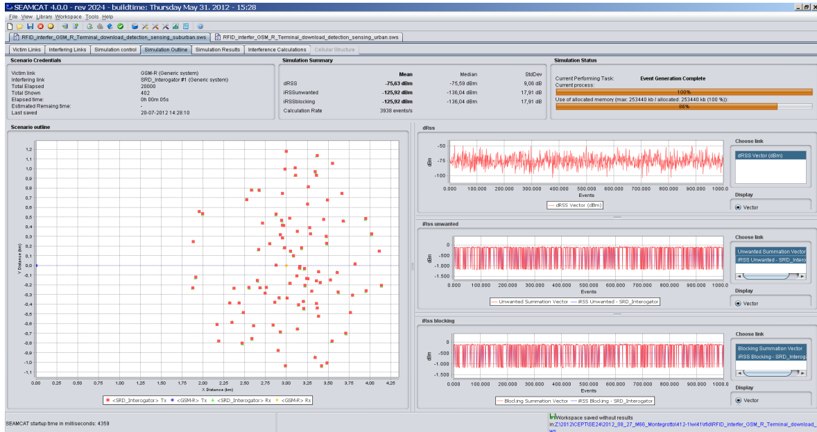
Figure 70: SEAMCAT simulation of RFID downlink sensing scenario
