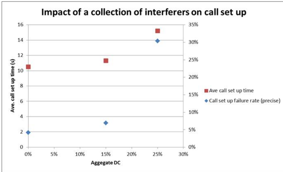
Figure 51: Impact of a collection of interferers on call set up
