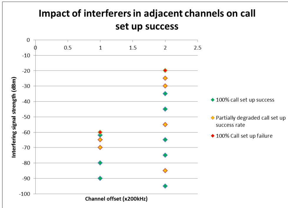
Figure 53: Detailed measurements of the impact of a 100% DC interferer in adjacent channels on call set up success (wanted signal -91dBm)
