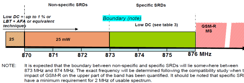
Figure 2: Tentative band plan for 870-876 MHz originally proposed in TR 102 649-2 [1]
