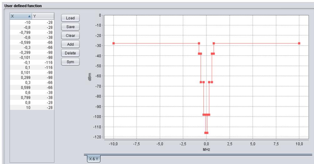
Figure 19: Receiver blocking mask GSM BS
