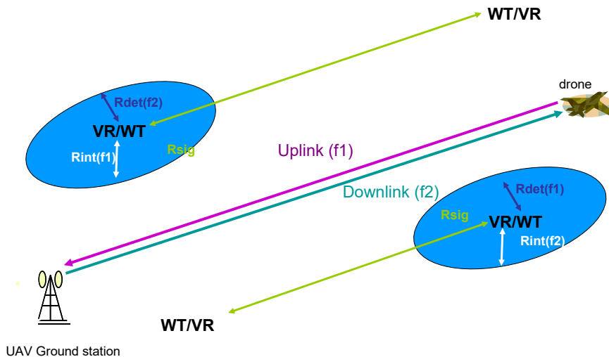
Figure 47: Illustration of scenario that assumes UAS with FDD
