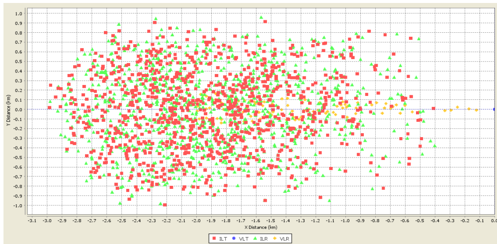
Figure 9: Example of SEAMCAT simulation window: SRD to ER-GSM
