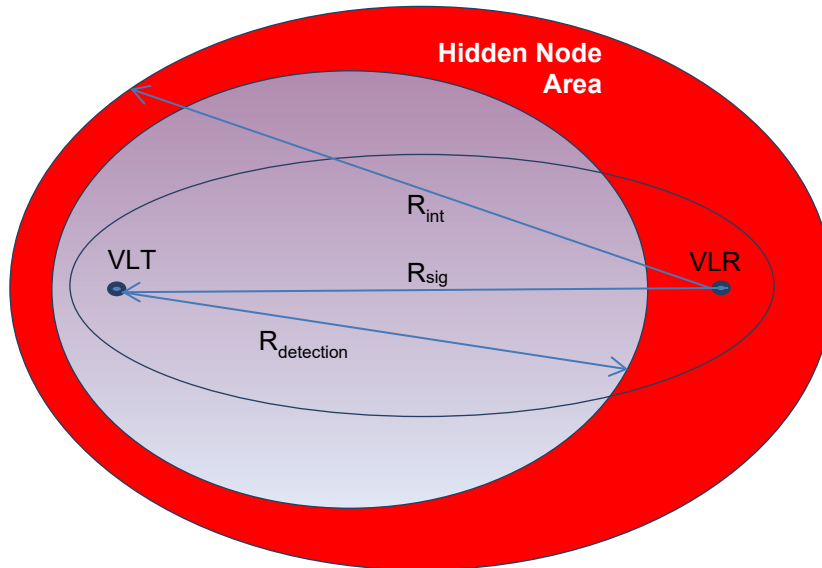
Figure 41: Illustration of DAA sensing deficiency (Hidden Node)
