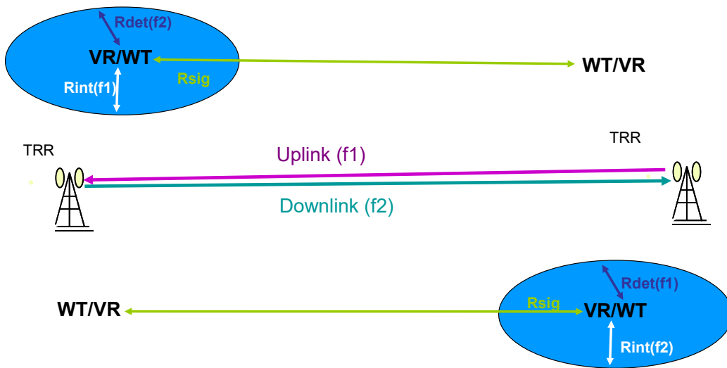
Figure 46: Illustration of scenario that assumes TRR with FDD
