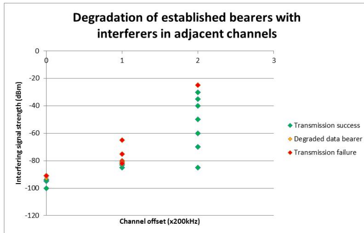
Figure 52: Detailed measurements of the impact of a 100% DC interferer in adjacent channels on bearer transmission reliability (wanted signal -91dBm)
