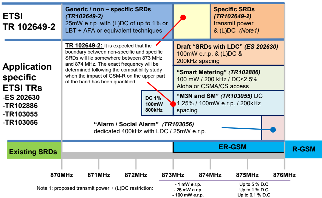
Figure 37: The summary of the updated SRdocs outlining SRD requirements in the band 870-876 MHz
