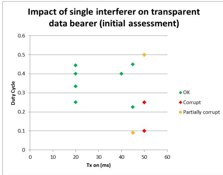
Figure 48: Impact of a single interferer on a transparent data bearer (initial assessment)
