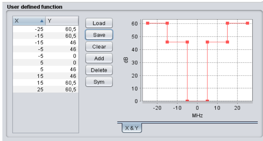
Figure 22: ACS LTE BS
