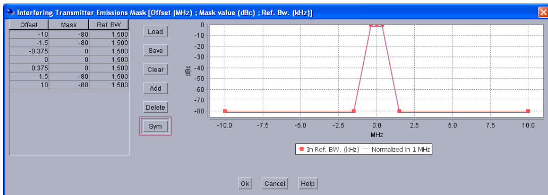
Figure 24: Unwanted emissions mask of TRR (ref. STANAG-4212 [18])
