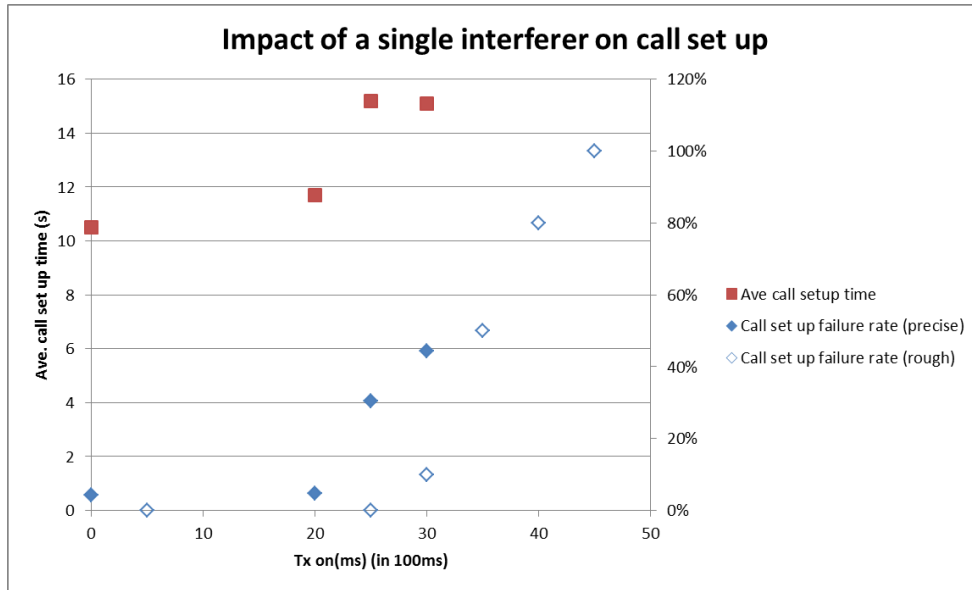
Figure 50: Impact of a single interferer on call set up
