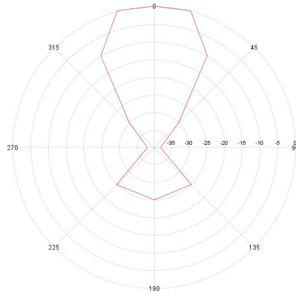
Figure 69: Horizontal antenna pattern of RFID Type 2 antenna
