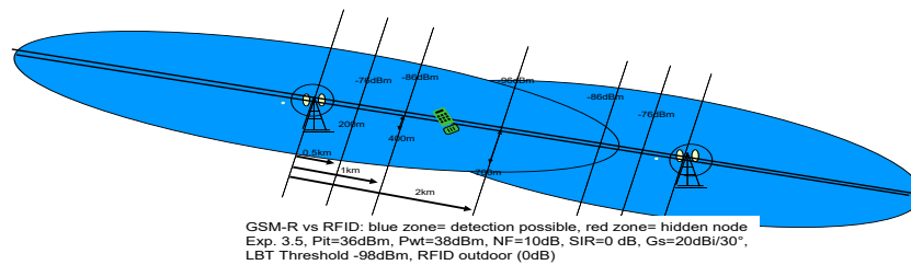
Figure 68: Figure 59: Hidden nodes (red areas) and detection areas (blue), RFID outdoor
