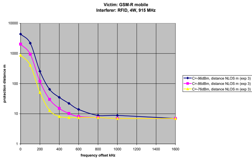
Figure 57: Protection distance between RFID interrogator and ER-GSM mobile under NLOS conditions
