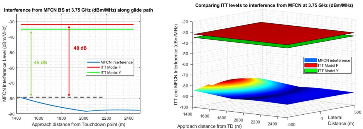
Figure 126: Comparing the ITT levels with the MFCN emissions at 3.75 GHz
