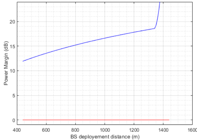
Figure 44: Power margin (dB) as a function of the BS deployment distance (m) within the runway axis, adjacent band non-AAS case
