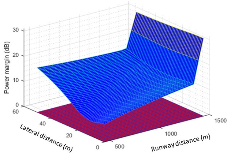
Figure 35: Power margin (dB) as a function of the BS deployment distance (m) along the runway axis D_{BS} and lateral axis L_{BS} for Adjacent-band non-AAS
