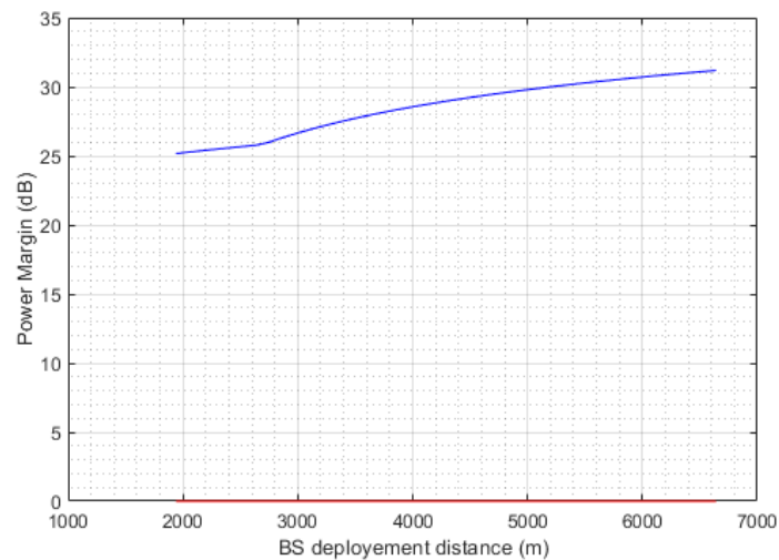
Figure 48: Power margin (dB) as a function of the BS deployment distance (m) within the runway axis, in-band non-AAS case
