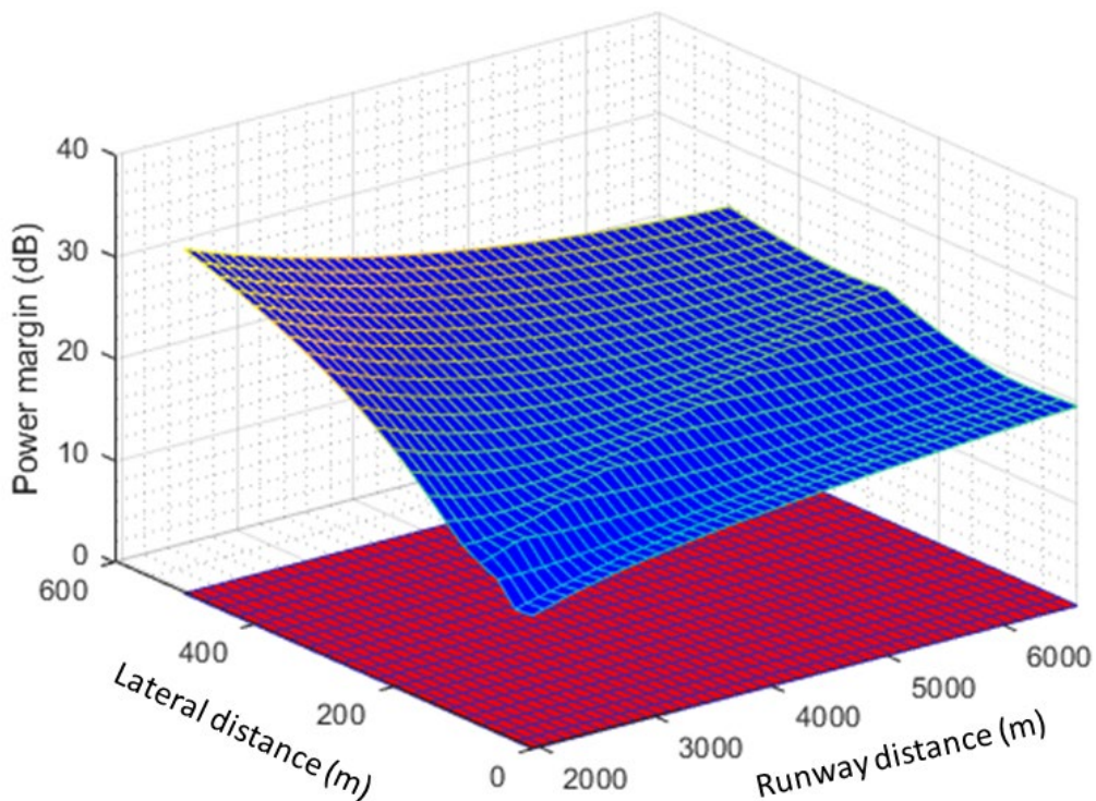
Figure 40: Power margin (dB) as a function of the BS deployment distance (m) along the runway axis D_{BS} and lateral axis L_{BS} for non-AAS (in-band case)
