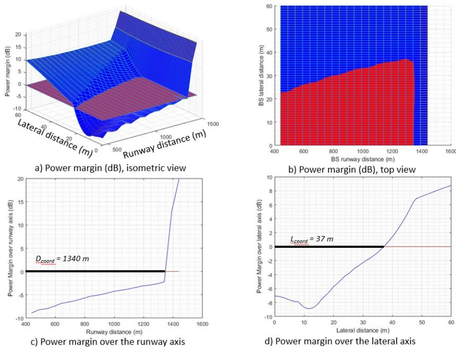
Figure 31: Power margin (dB) as a function of the BS deployment distance (m) along the runway axis D_{BS} and lateral axis L_{BS} for 4x4 AAS for BEM derived from ETSI TS 138 104, section 9.7.4
