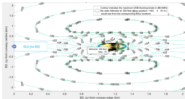
Figure 75: Contour plot showing the maximum OOB blocking levels in dBm/MHz the Altimeter would see from the corresponding \Delta x , \Delta y BS location from the RP. The result is for Altimeter at 200 feet (1163, 0, 61) meters, and with up to \pm 15 degrees roll. Medium power AAS BS with 6 m height operating at f_c = 4.15 GHz
