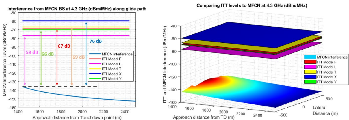
Figure 127: Comparing the ITT levels with the MFCN in the unwanted emissions at 4.3 GHz
