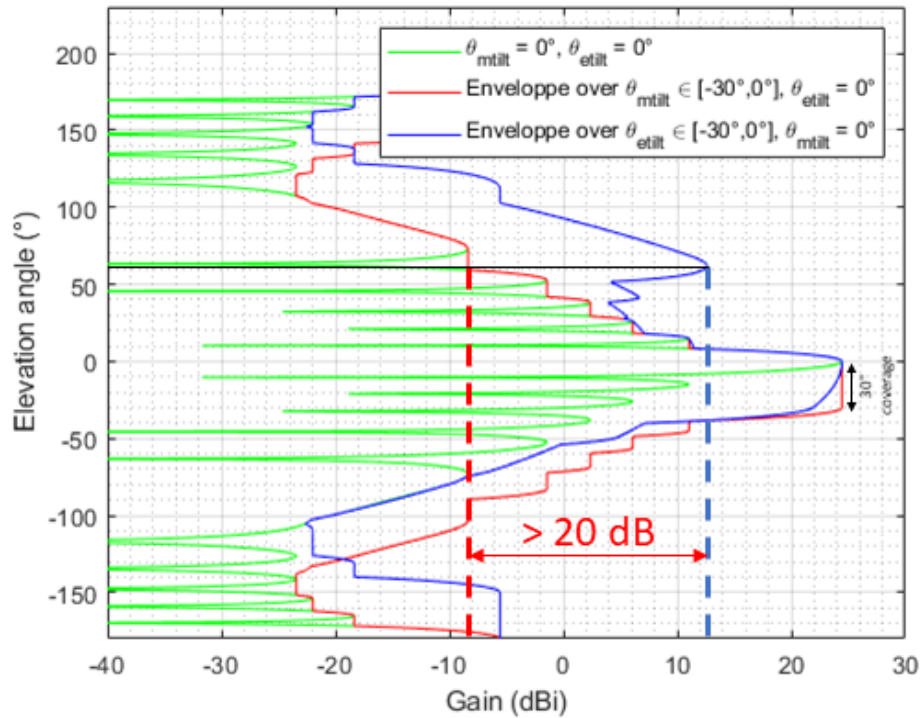
Figure 50: Difference of AAS radiation pattern envelope when considering either mechanical tilts or electronic tilts
