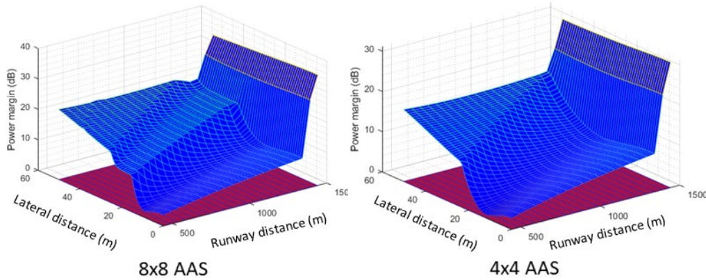
Figure 26: Power margin (dB) as a function of the BS deployment distance (m) along the runway axis D_{BS} and lateral axis L_{BS} for 8x8 AAS and 4x4 AAS cases
