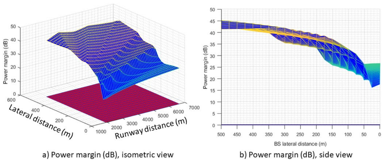
Figure 36: Power margin (dB) as a function of the BS deployment distance (m) along the runway axis D_{BS} and lateral axis L_{BS} for 8x8 AAS (in-band case)
