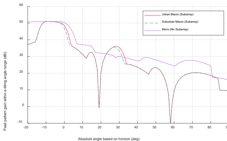
Figure 172: Enveloped e.i.r.p. of BS according to AAS configurations with and without subarray
