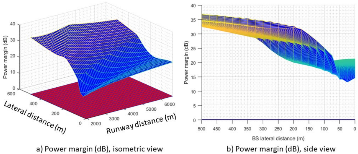
Figure 39: Power margin (dB) as a function of the BS deployment distance (m) along the runway axis D_{BS} and lateral axis L_{BS} for 4x4 AAS (adjacent-band case)
