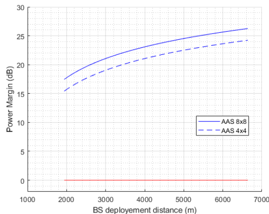
Figure 45: Power margin (dB) as a function of the BS deployment distance (m) within the runway axis, AAS 8x8 and 4x4 cases
