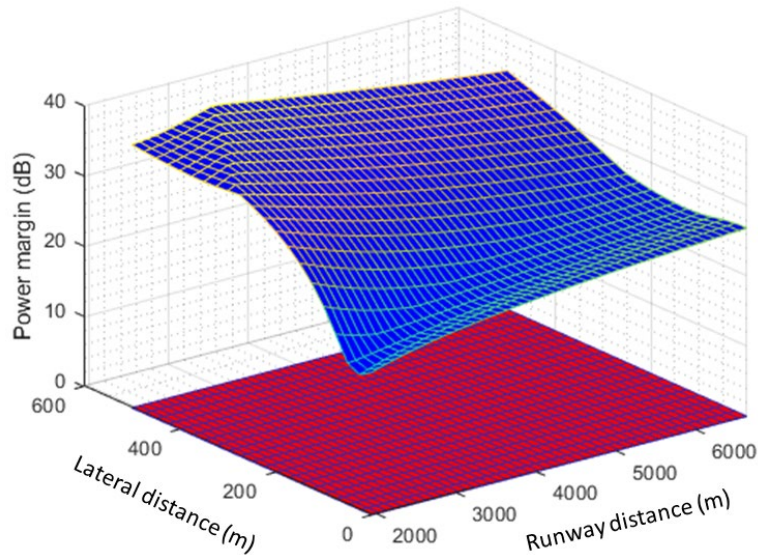
Figure 41: Power margin (dB) as a function of the BS deployment distance (m) along the runway axis D_{BS} and lateral axis L_{BS} for non-AAS (adjacent-band case)
