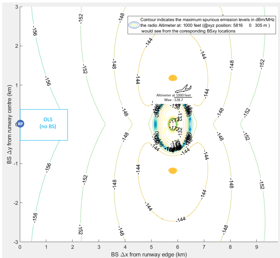
Figure 72: Contour plot showing the maximum spurious emission levels in dBm/MHz the Altimeter would see from the corresponding \Delta x , \Delta y BS location from the RP. The result is for Altimeter at 1000 feet (5816, 0, 305) and with up to \pm 15 degrees roll. For macro urban AAS BS with 35 m height
