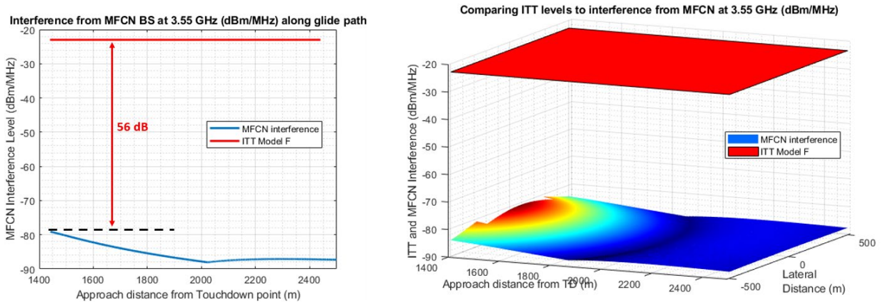
Figure 125: Comparing the ITT levels with the MFCN emissions at 3.55 GHz
