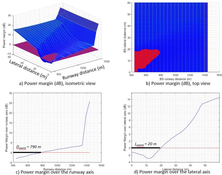
Figure 33: Power margin (dB) as a function of the BS deployment distance (m) along the runway axis D_{BS} and lateral axis L_{BS} for 4x4 AAS for BEM derived from ETSI TS 138 104 section 9.7.4 reduced by 6 dB
