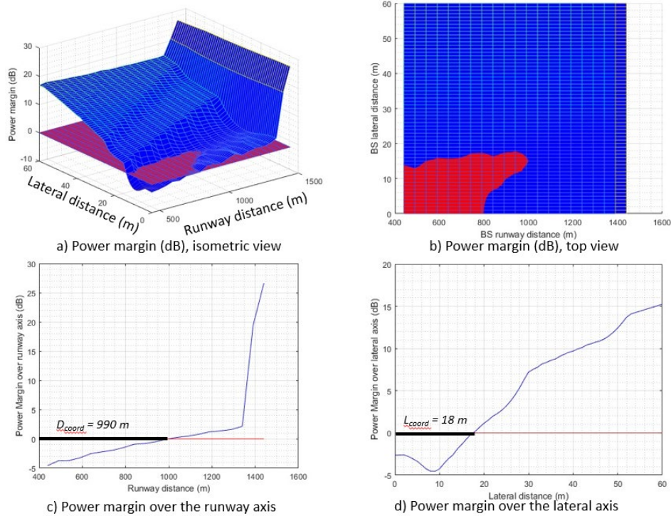
Figure 28: Power margin (dB) as a function of the BS deployment distance (m) along the runway axis and lateral axis for 8x8 AAS
