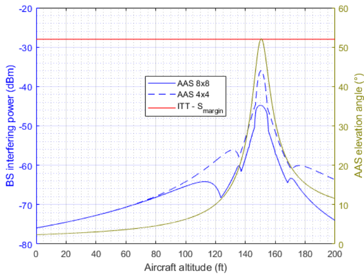
Figure 27: Base station interfering power (dBm) as a function of the aircraft height (feet) for a base station deployed at D_{BS} = 1000 m L_{BS} = 30 m
