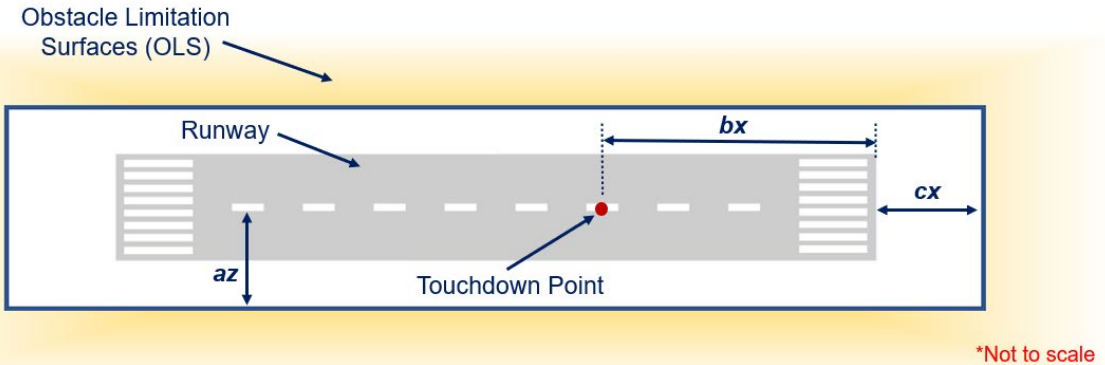
Figure 145: The runway
