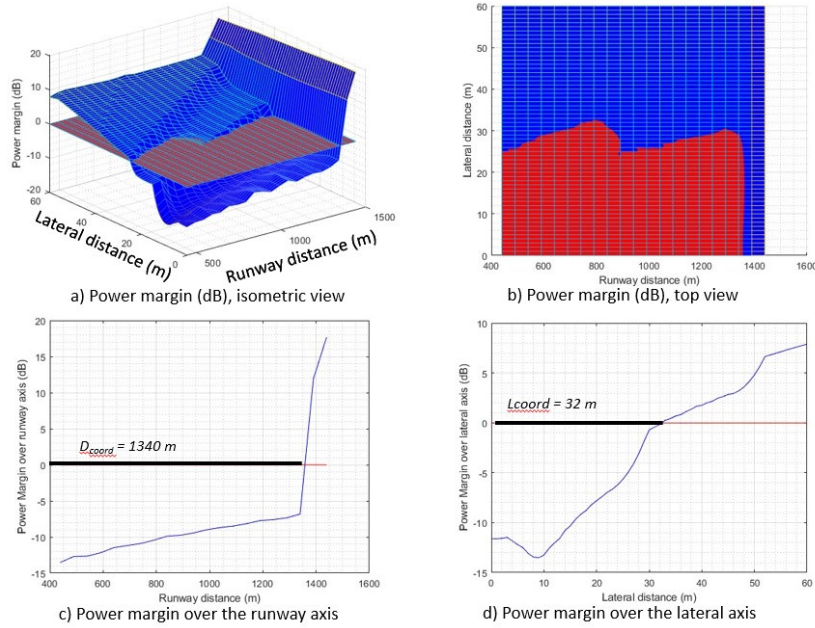
Figure 30: Power margin (dB) as a function of the BS deployment distance (m) along the runway axis D_{BS} and lateral axis L_{BS} for 8x8 AAS for BEM derived from ETSI TS 138 104, section 9.7.4
