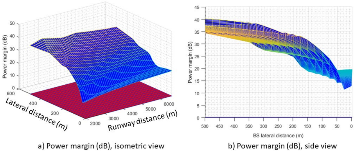
Figure 38: Power margin (dB) as a function of the BS deployment distance (m) along the runway axis D_{BS} and lateral axis L_{BS} for 8x8 AAS (adjacent-band case)
