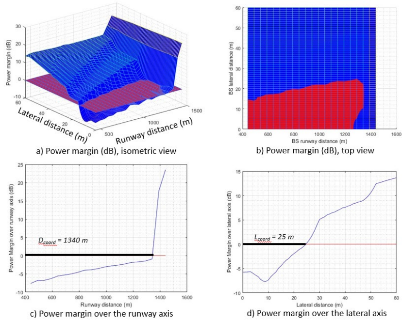
Figure 32: Power margin (dB) as a function of the BS deployment distance (m) along the runway axis D_{BS} and lateral axis L_{BS} for 8x8 AAS for BEM derived from ETSI TS 138 104 section 9.7.4 reduced by 6 dB
