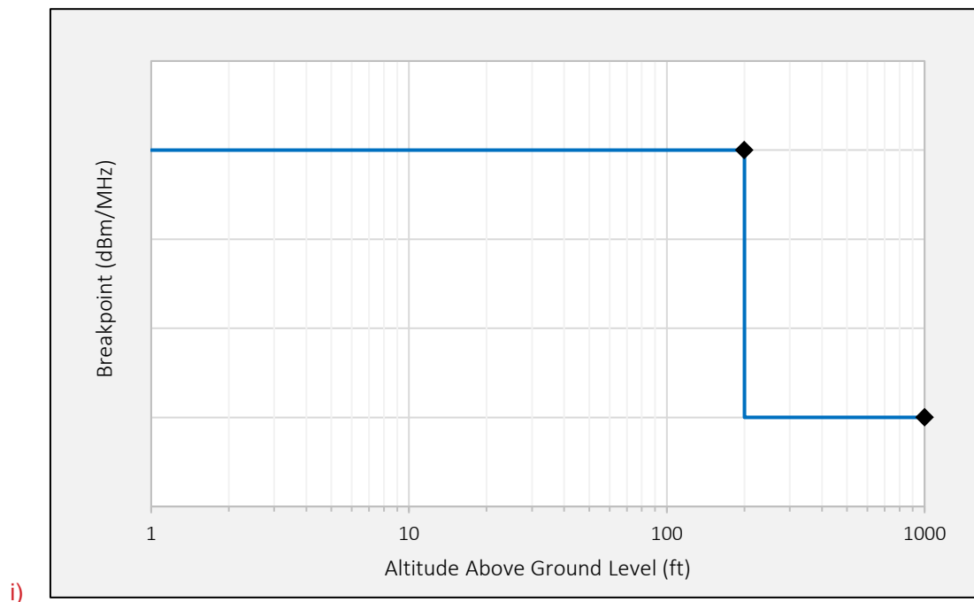
Figure 58: Example of stair-step interpolation and extrapolation
