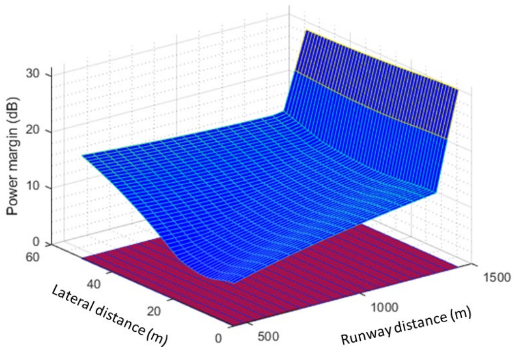
Figure 34: Power margin (dB) as a function of the BS deployment distance (m) along the runway axis D_{BS} and lateral axis L_{BS} for In-band non-AAS
