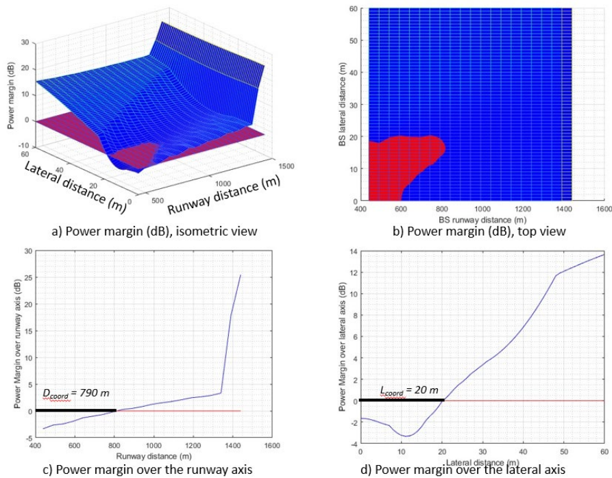
Figure 29: Power margin (dB) as a function of the BS deployment distance (m) along the runway axis and lateral axis for 4x4 AAS
