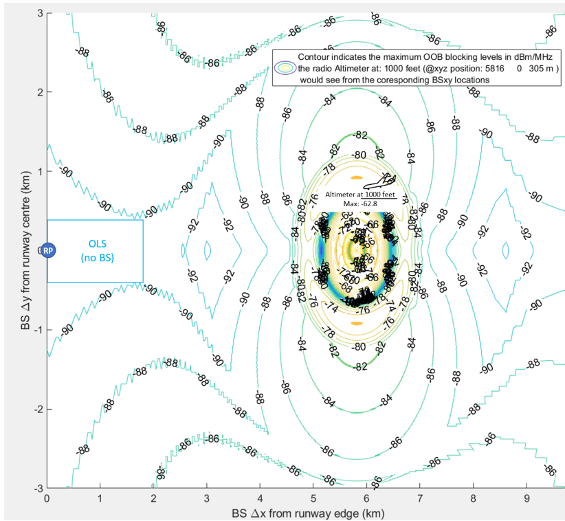
Figure 71: Contour plot showing the maximum OOB blocking levels in dBm/MHz the Altimeter would see from the corresponding \Delta x , \Delta y BS location from the RP. The result is for Altimeter at 1000 feet (5816, 0, 305) and with up to \pm 15 degrees roll. For macro rural AAS BS with 35 m height
