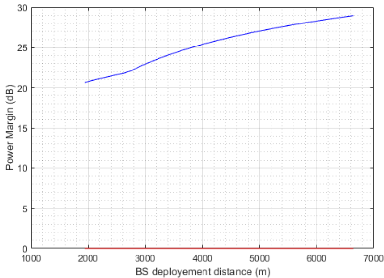
Figure 47: Power margin (dB) as a function of the BS deployment distance (m) within the runway axis, in-band non-AAS case
