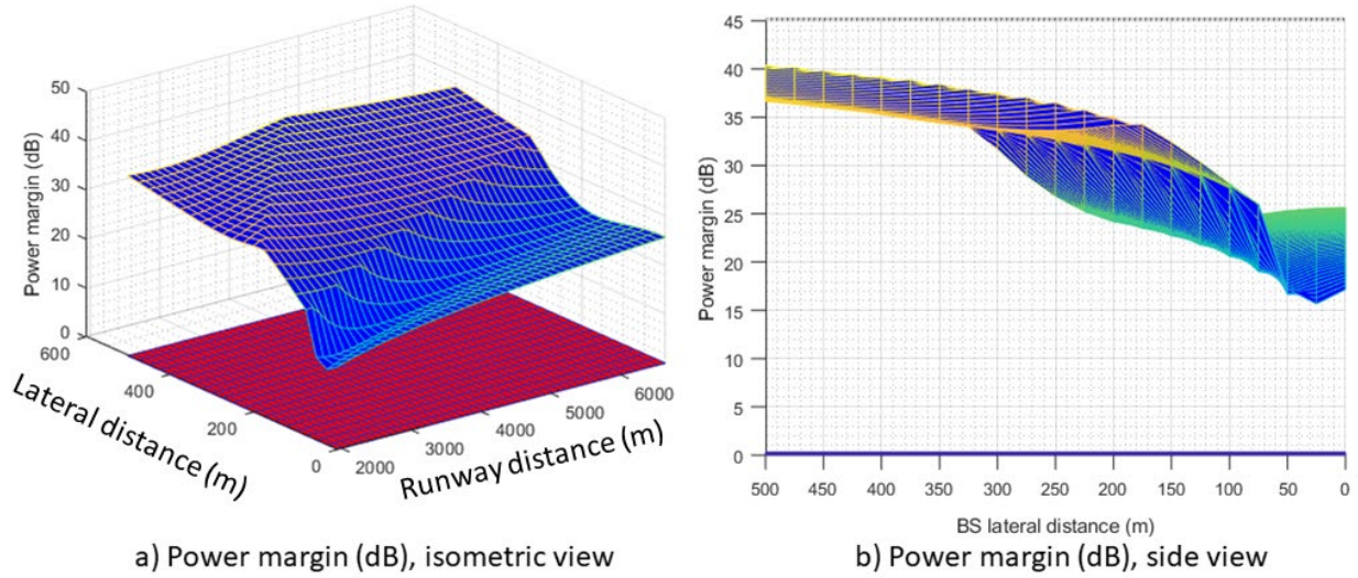
Figure 37: Power margin (dB) as a function of the BS deployment distance (m) along the runway axis D_{BS} and lateral axis L_{BS} for 4x4 AAS (in-band case)
