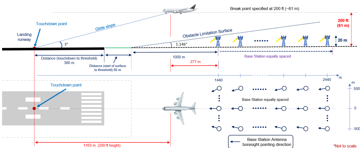
Figure 117: Interference scenario
