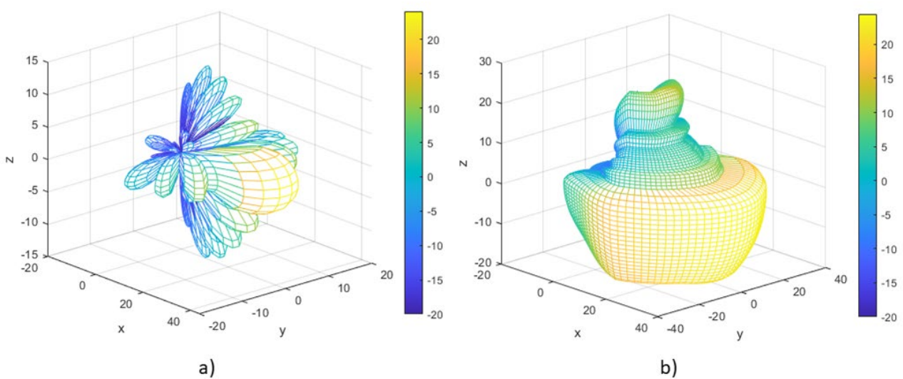
Figure 51: AAS radiation pattern a) No envelope ( \varphi_{escan} = \theta_{etilt} = 0^\circ ) b) with envelope ( \theta_{etilt} \in [-30^\circ, 0] , \varphi_{escan} \in [-60^\circ, 60^\circ] )
