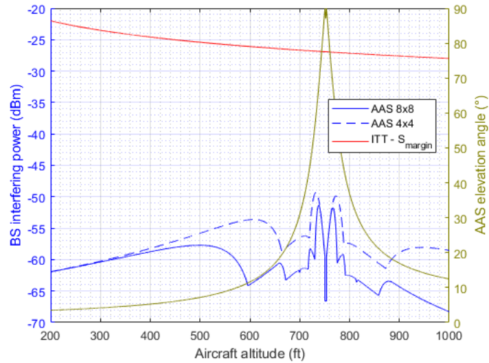
Figure 46: Base station interfering power (dBm) as a function of the aircraft height (feet) for a base station deployed at D_{BS} = 5000 m within the runway axis
