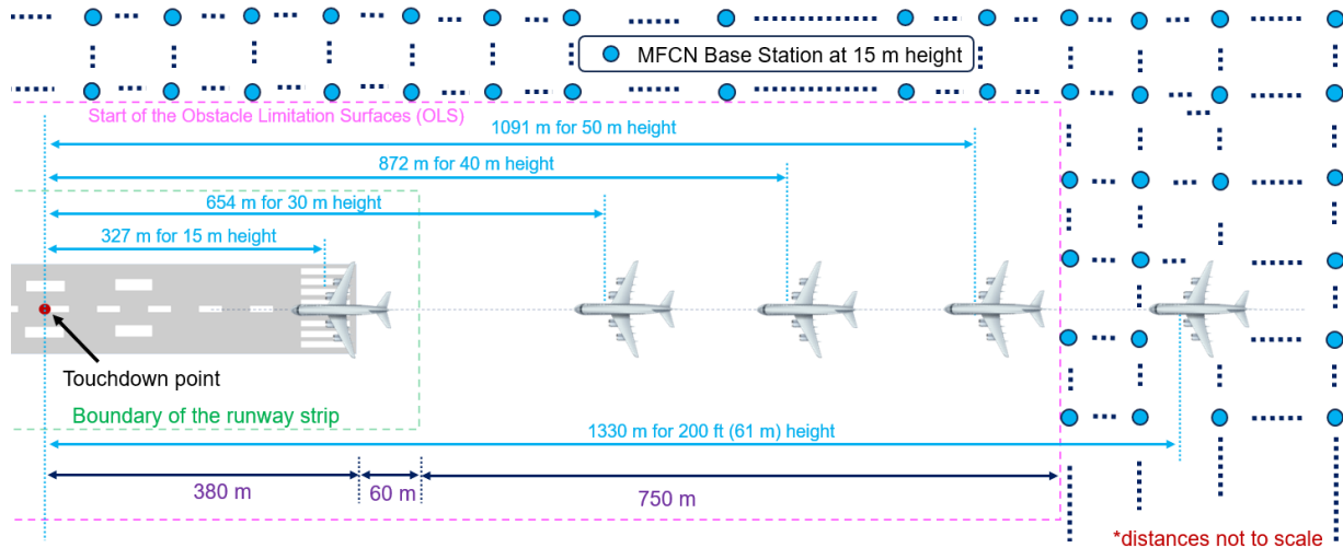
Figure 141: Interference scenario
