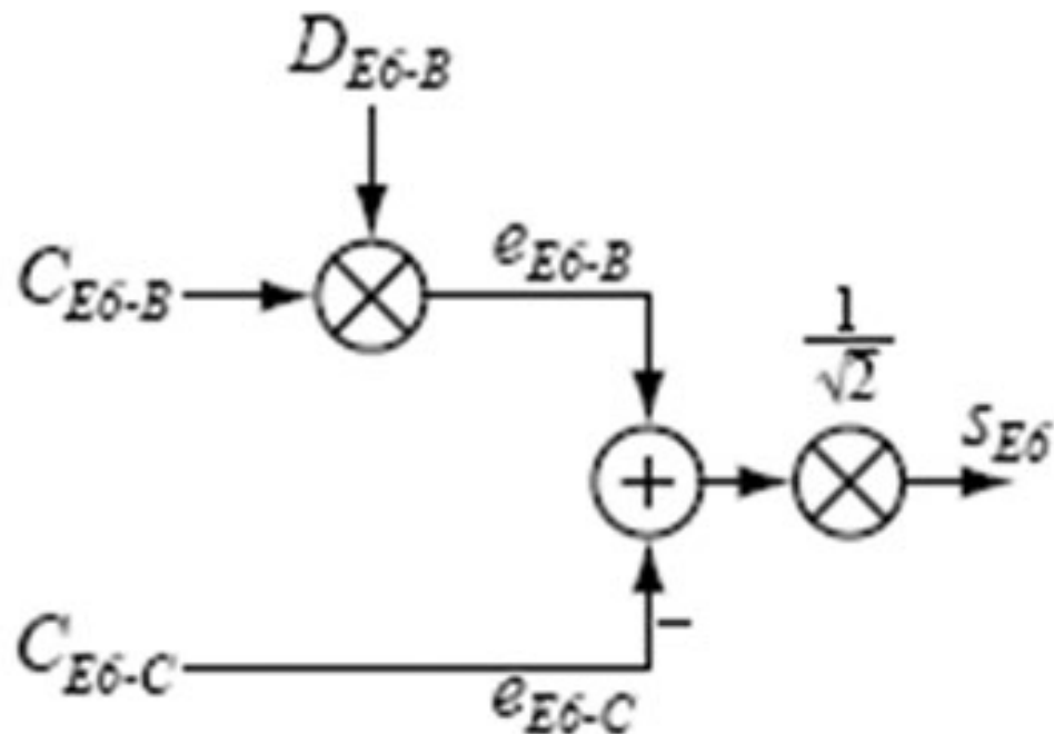
Figure 2: Multiplexing of the Galileo E-6B+C signal
