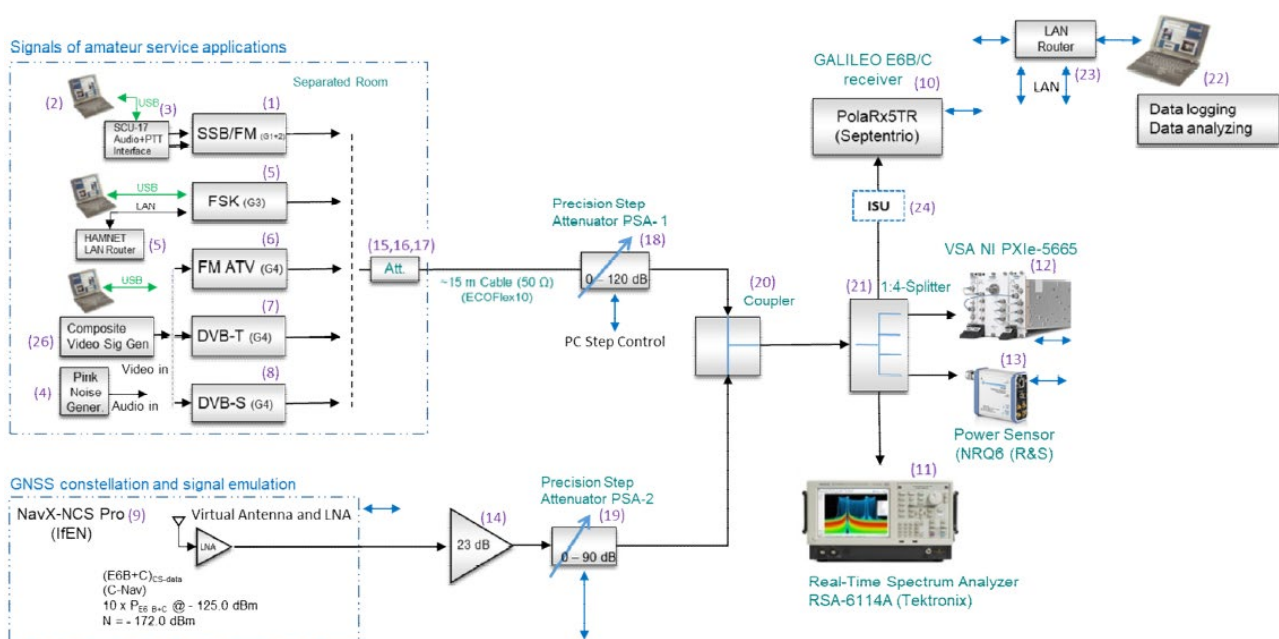
Figure 14: Measurement setup
