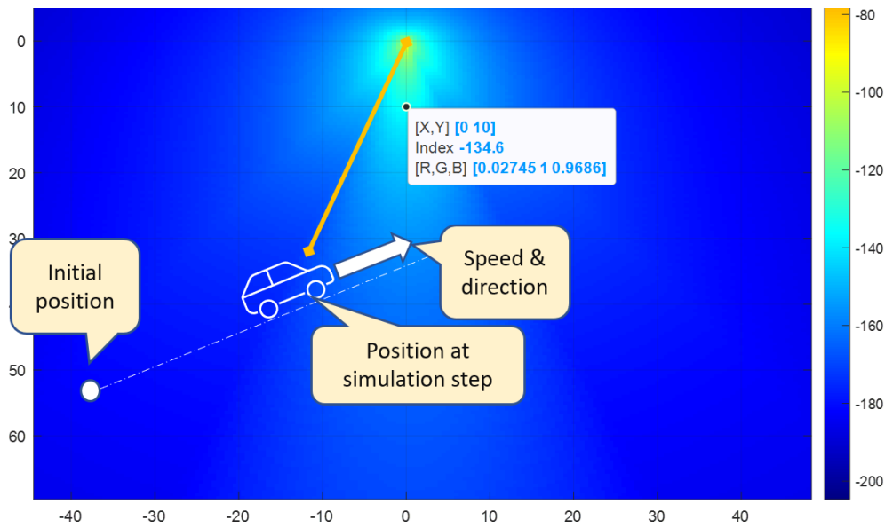
Figure 10: Mobile RNSS receiver simulation scenario
