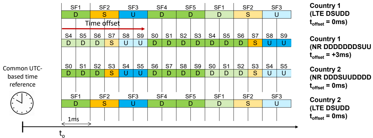
Figure 2: Aligned of LTE and LTE-compatible frame structures over the air
