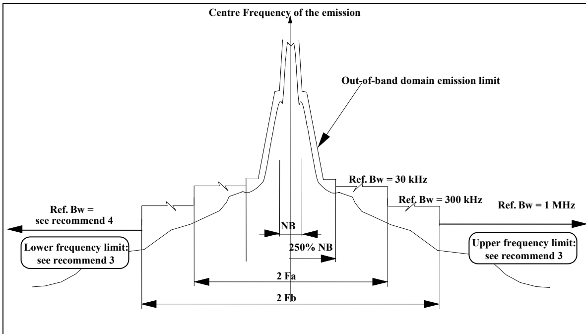
Figure 2: Specific mask for spurious domain emissions with reference bandwidths for BWA systems operating between 1 GHz and 6 GHz (see Table 5)
