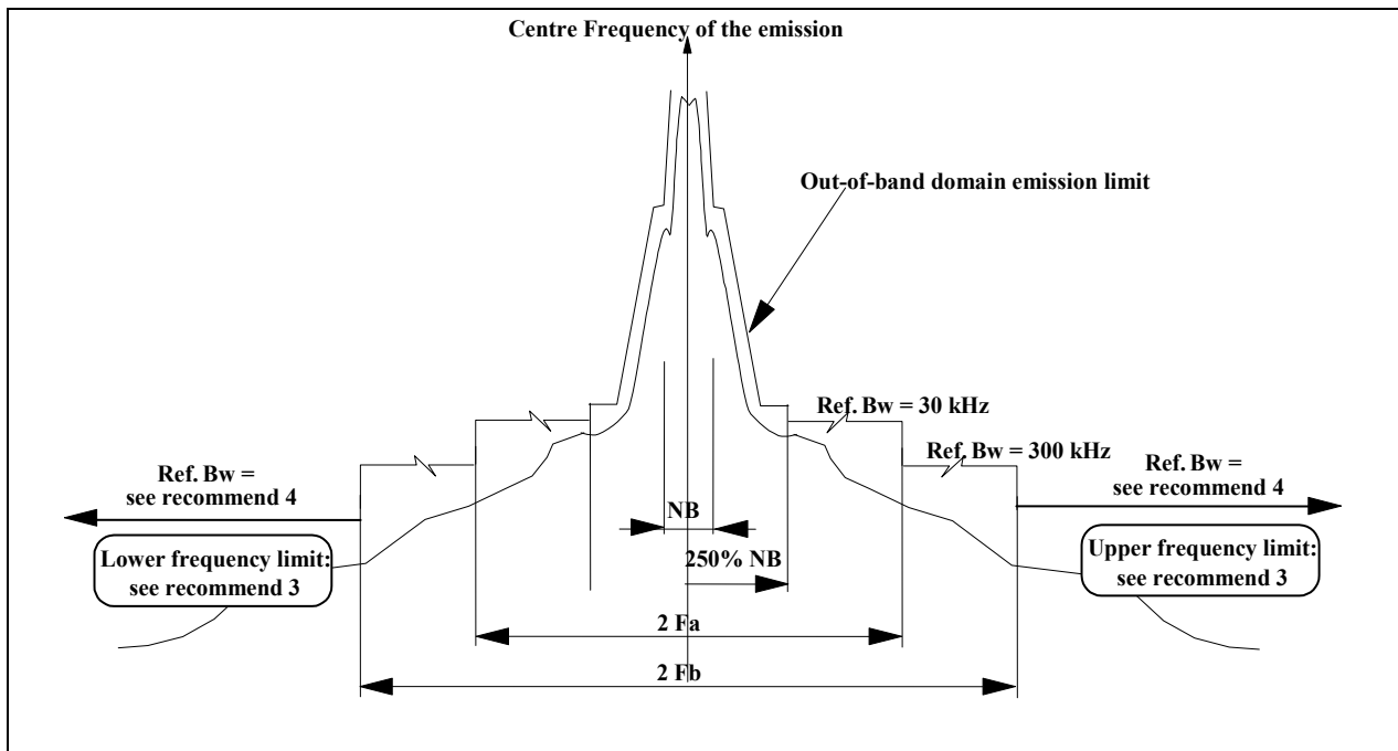
Figure 5: Specific mask for spurious domain emissions with reference bandwidths for mobile services operating above 1 GHz (see Table 8)
