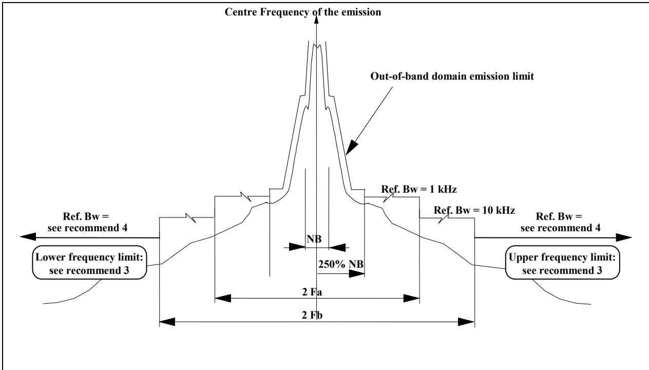
Figure 4: Specific mask for spurious domain emissions with reference bandwidths for mobile services operating between 30 MHz and 1 GHz (see Table 7)
