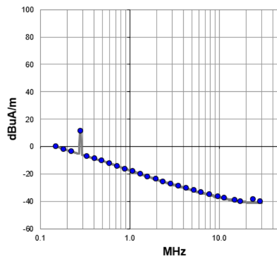
Figure 47: 10 m Test Distance, SAC, 0 degrees, Receive Antenna Parallel to Charger
