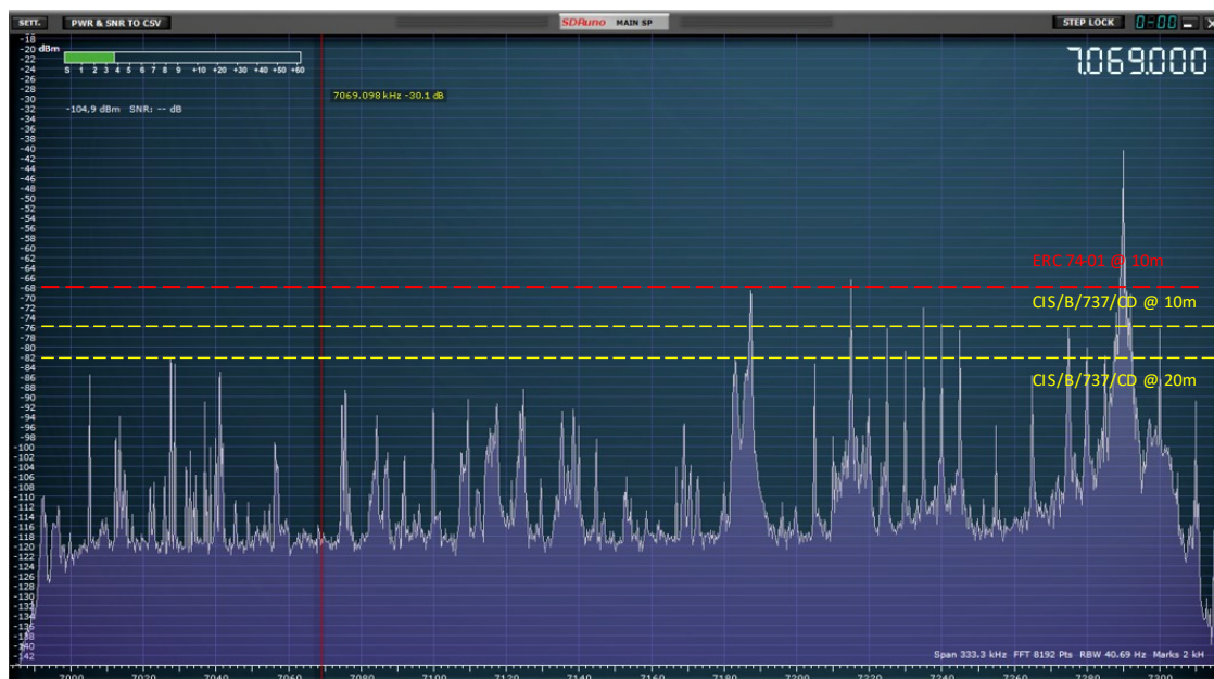
Figure 16: 7 MHz spectrum – late afternoon March 2021
