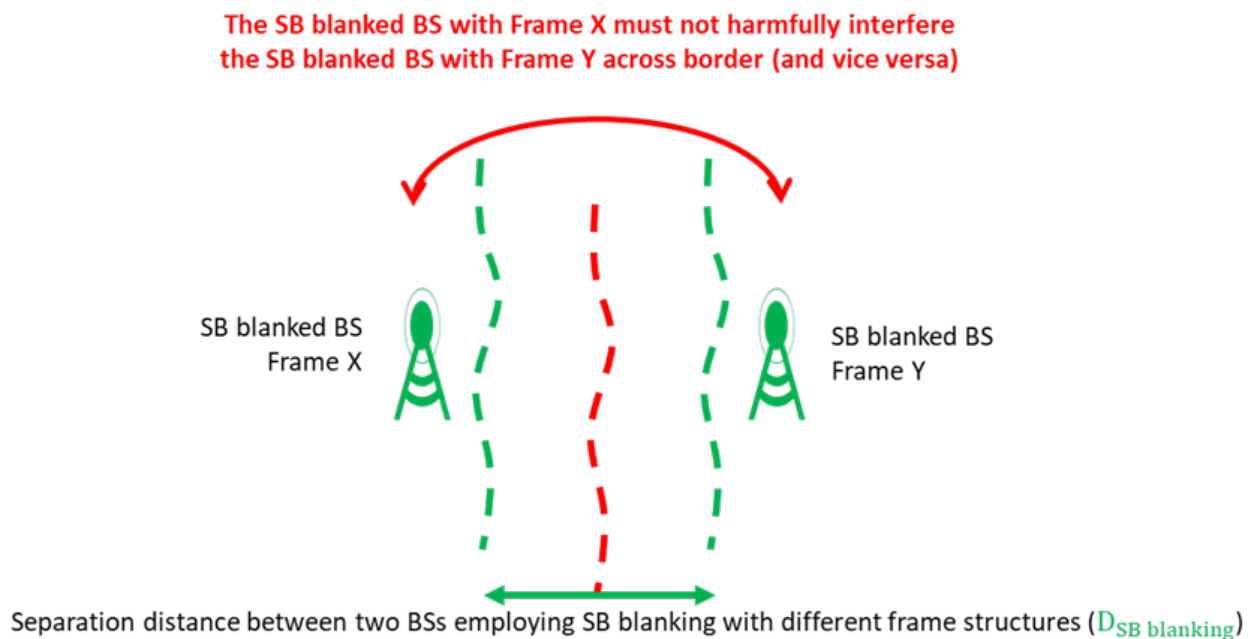
Figure 12 : The separation distance in case of unsynchronised operation with a common phase clock reference with sub-band blanking
