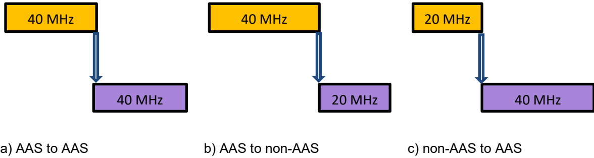
Figure 24: Adjacent channel DL to UL
