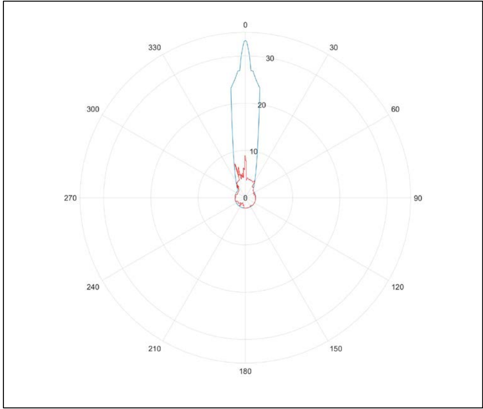
Figure 31: Protection contours
