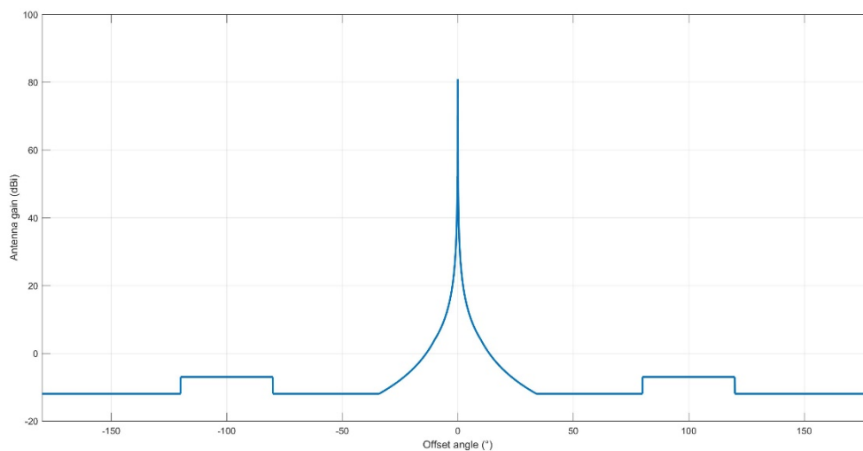
Figure 12: RAS antenna pattern (basic version)
