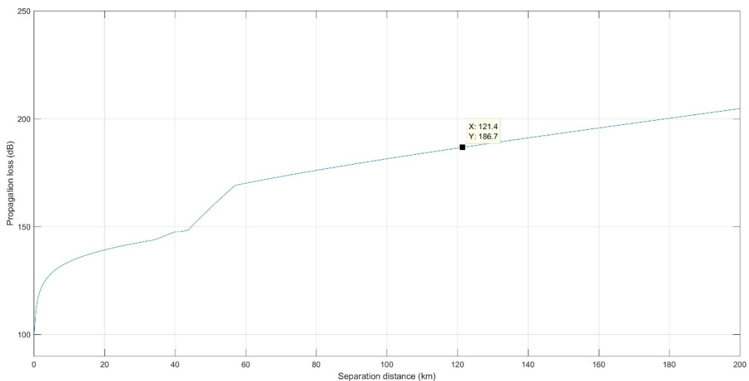
Figure 40: Recommendation ITU-R P.452 Propagation loss over flat terrain
