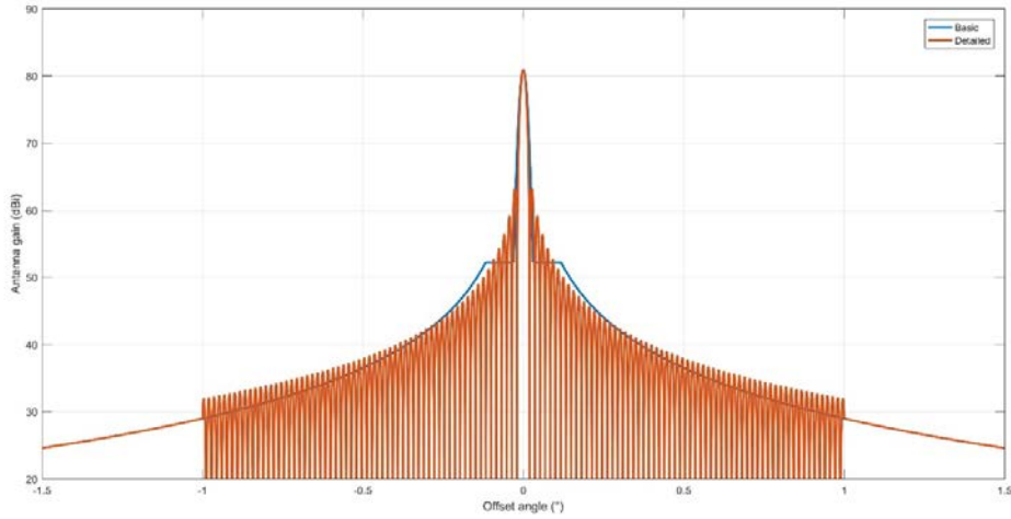
Figure 13: RAS antenna pattern (detailed version - zoomed around the main beam)
