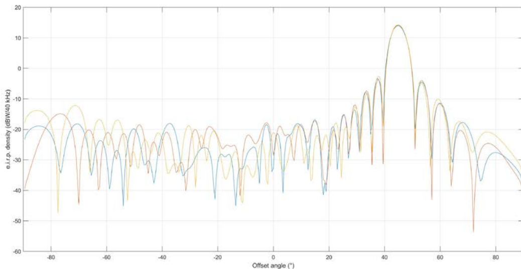
Figure 10: e.i.r.p. mask for the phased array antenna (dBW/(40 kHz)) for 45° pointing for three frequencies (14, 14.25 and 14.5 GHz)
