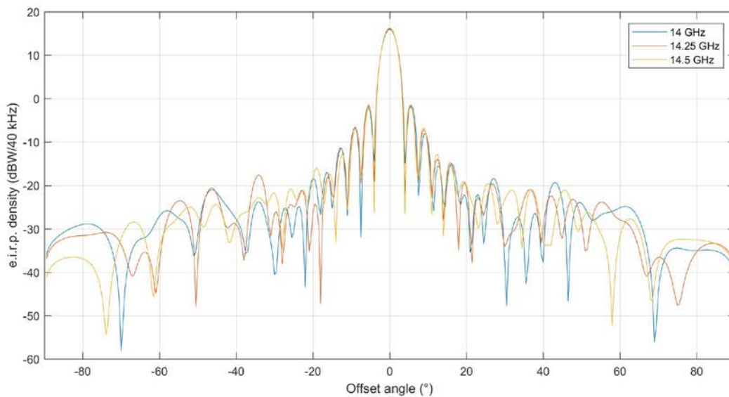
Figure 8: e.i.r.p. mask for the phased array antenna (dBW/(40 kHz)) for 90° pointing for three frequencies (14, 14.25 and 14.5 GHz)
