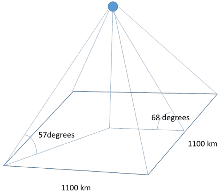
Figure 4: Determination of the minimum elevation angle
