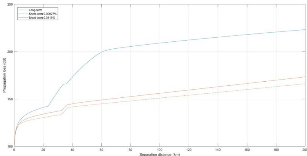
Figure 30: Recommendation ITU-R P.452 Propagation loss over flat terrain
