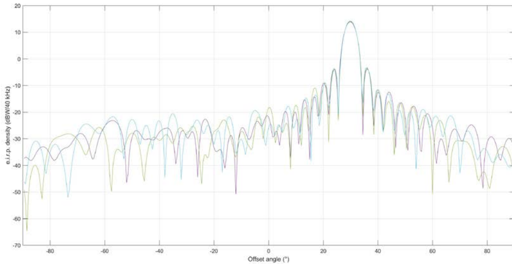
Figure 9: e.i.r.p. mask for the phased array antenna (dBW/(40 kHz)) for 120° pointing for three frequencies (14, 14.25 and 14.5 GHz)
