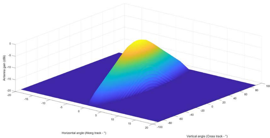
Figure 3: - 3 dB composite antenna aperture
