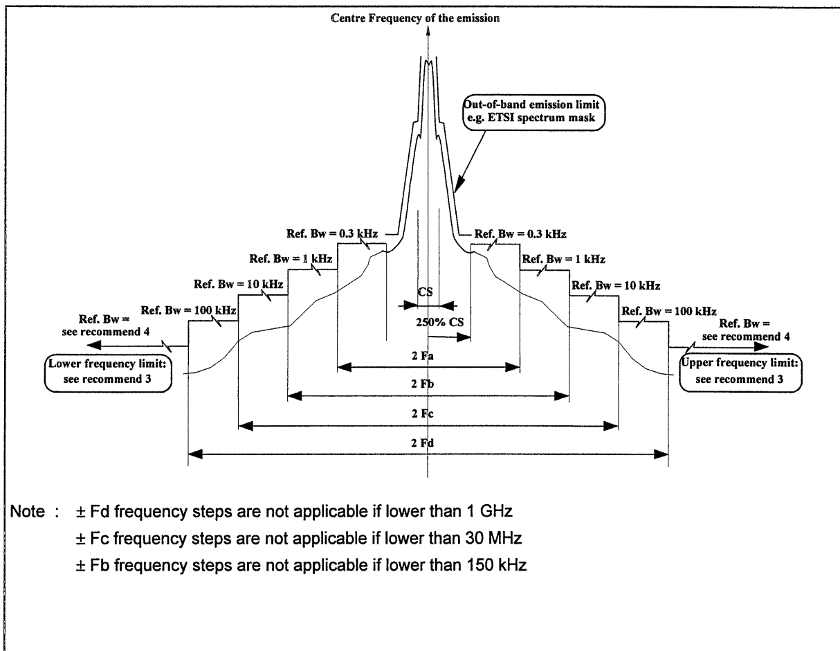
Fig. 1.1 : Specific spurious emissions limit mask (ref. to table 1.2)
