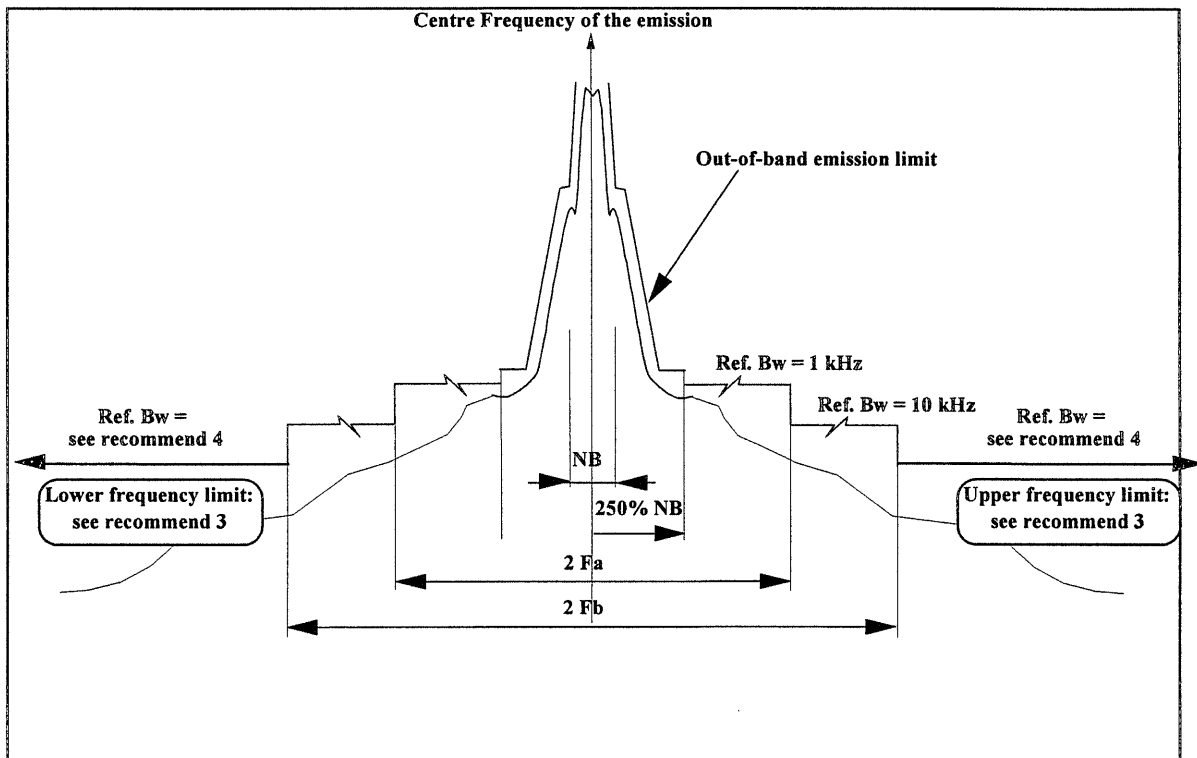
Fig. 2.1 : Specific spurious emissions mask for mobile service operating between 30 MHz and 1 GHz (refer table 2.2)
