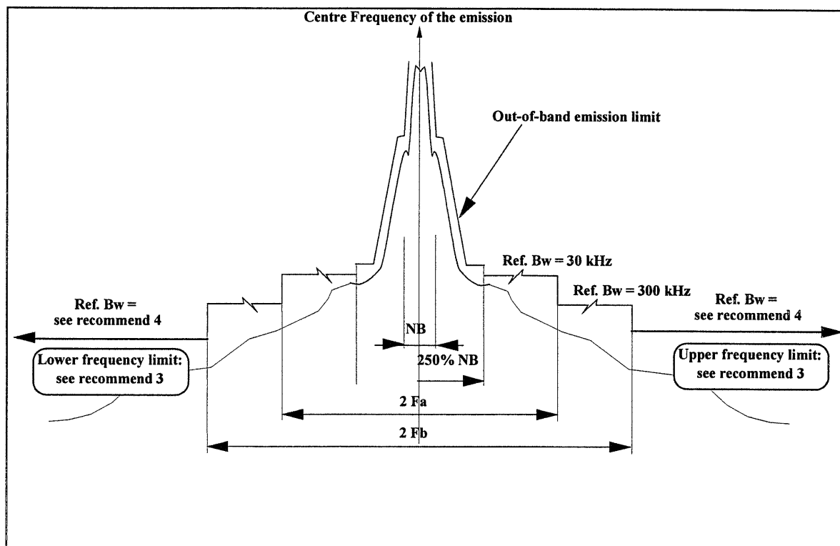
Fig. 2.2 : Specific spurious emissions limit mask for mobile service operating above 1 GHz (refer table 2.3)
