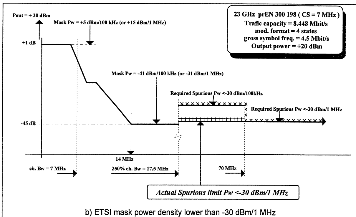
Fig. 1.2 : Examples of ETSI mask more stringent than the spurious emission limits in the reference BW (ref. to note to table 1.2)
