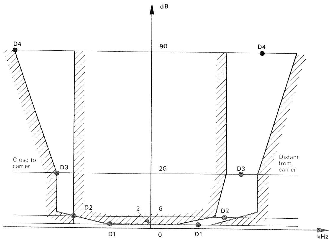
Figure 2 (T/R 20-04). Selectivity characteristic of the "receiver".
