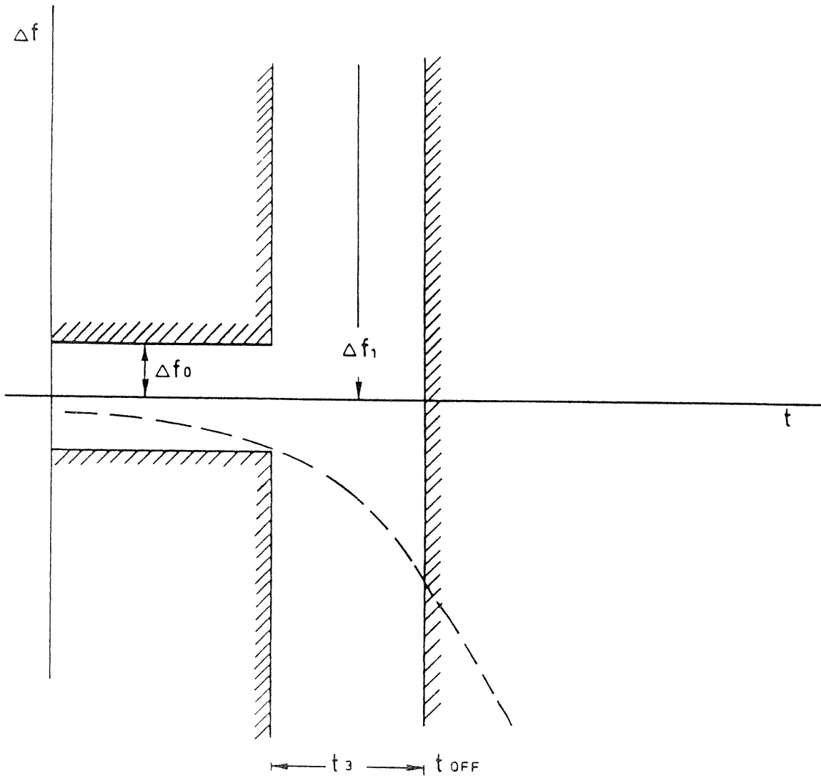
Figure B (T/R 20-04). Transient state at shut-down (Clauses B.1.2. and B.1.3.).
