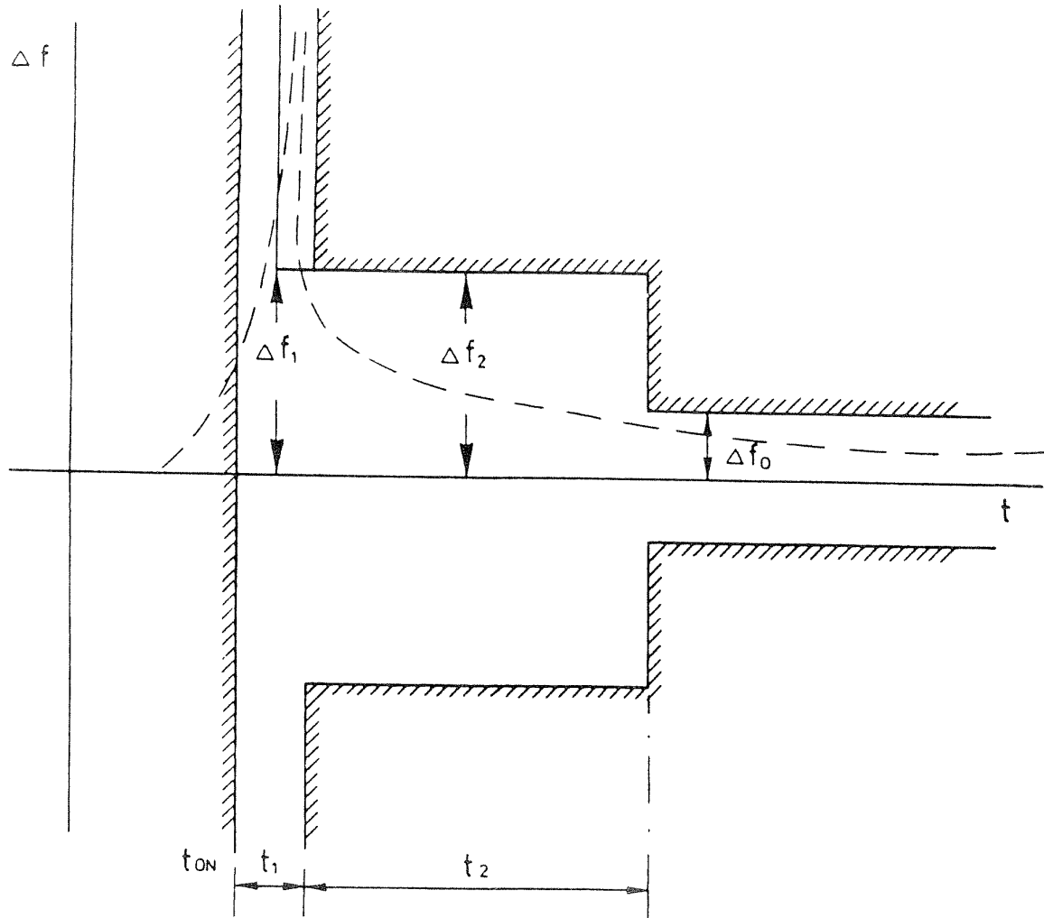
Figure A (T/R 20-04). Transient state at start-up (Clauses B.1.1. and B.1.3.).
