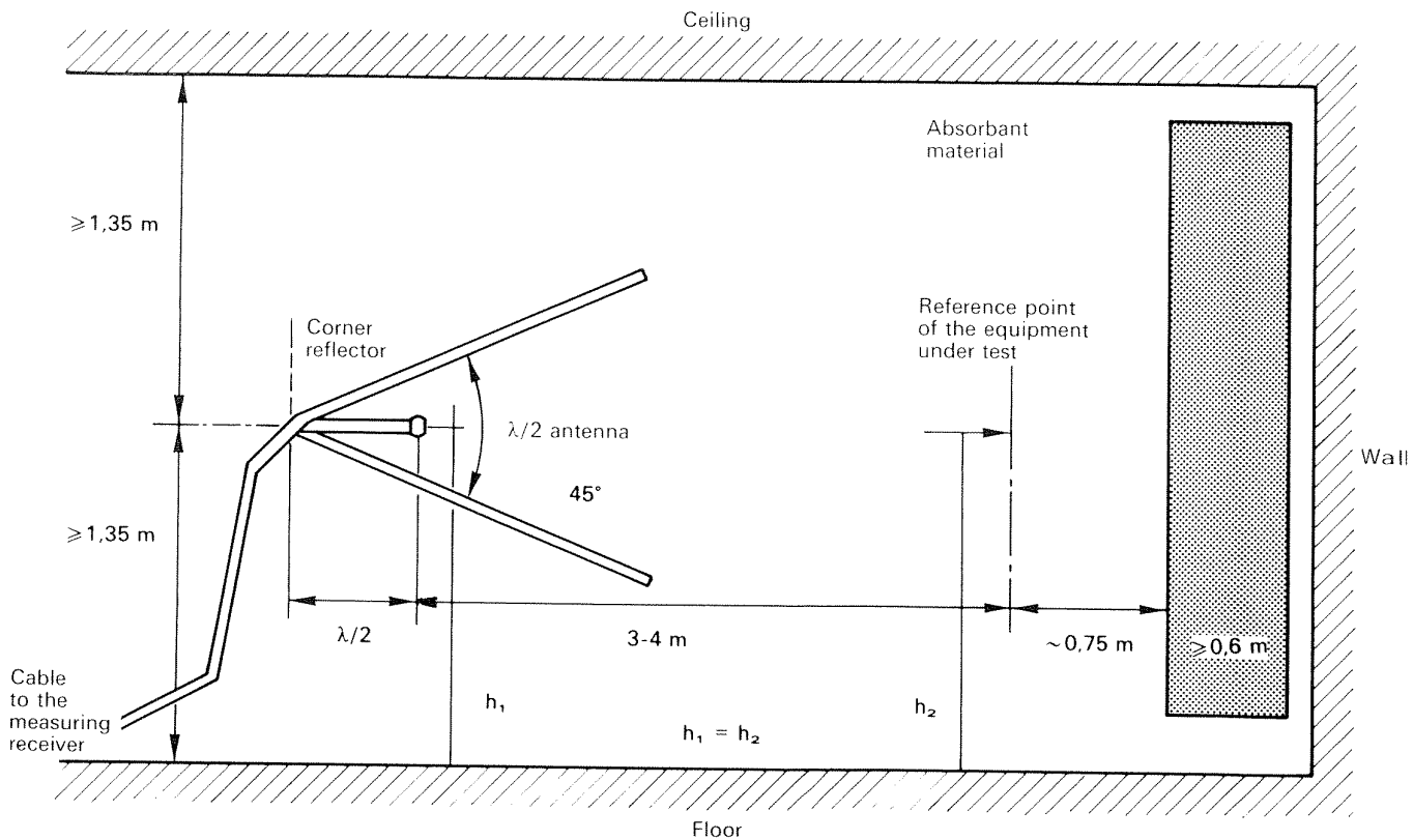
Figure 1 (T/R 20-04). Indoor site arrangement (shown for horizontal polarization).
