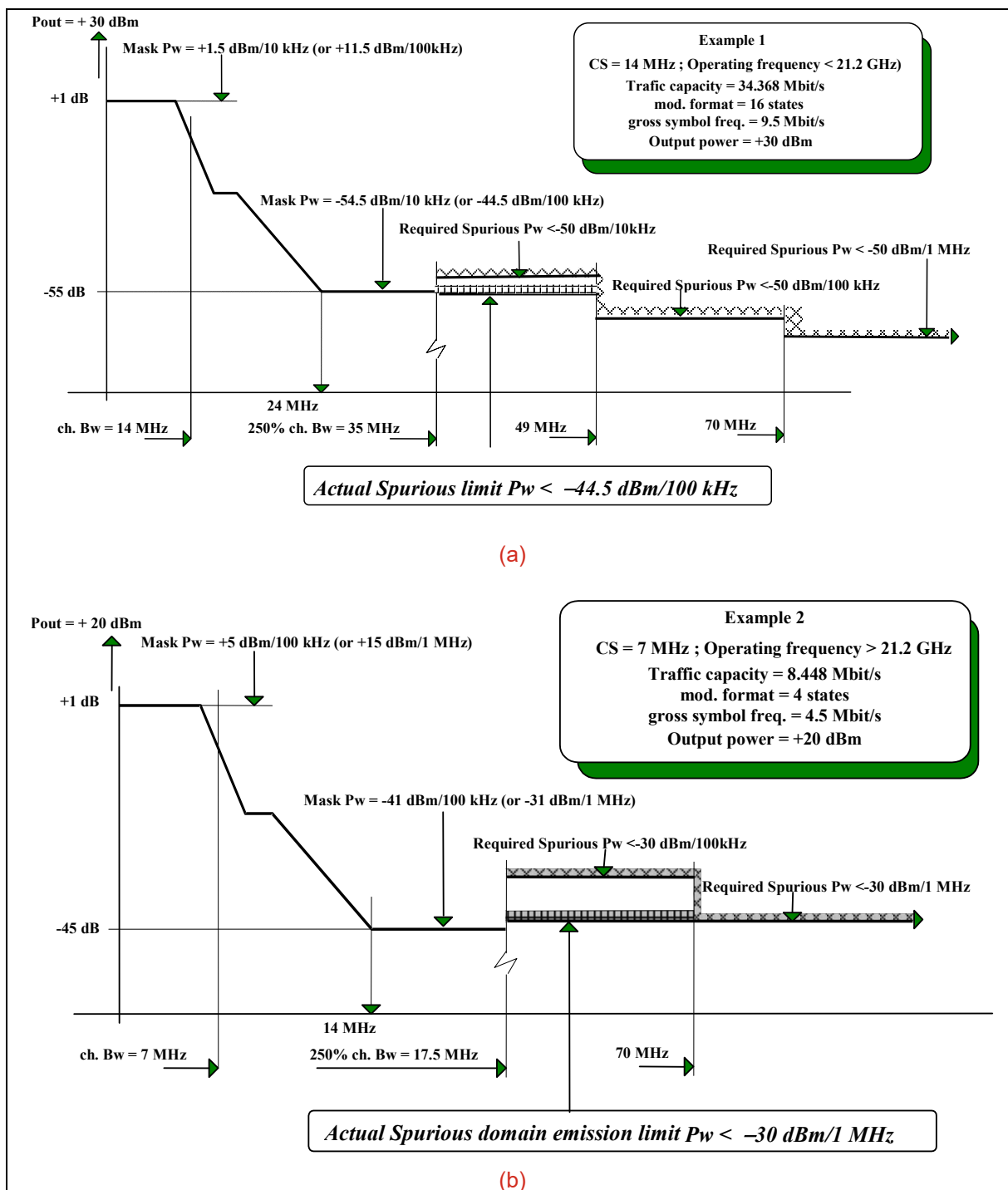
Figure 3: Examples of spectrum power density masks 6 being more stringent than the spurious domain emission limits in the reference bandwidth (refer to Note to Table 4)
