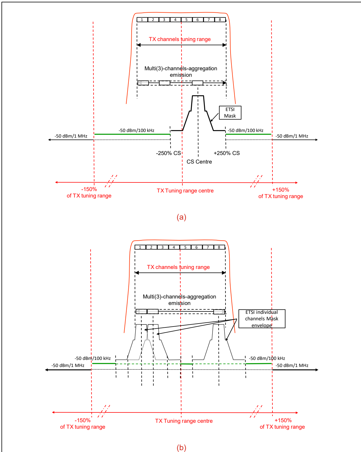
Figure 4: (a) Specific mask for spurious domain emissions for channel aggregation (single band/multiple channels port) systems operating below 21.2 GHz (example with 3 channels ) (b): Example with combined limits for channel aggregation (single band/multiple channels port) systems operating below 21.2 GHz (example with 3 channels)
