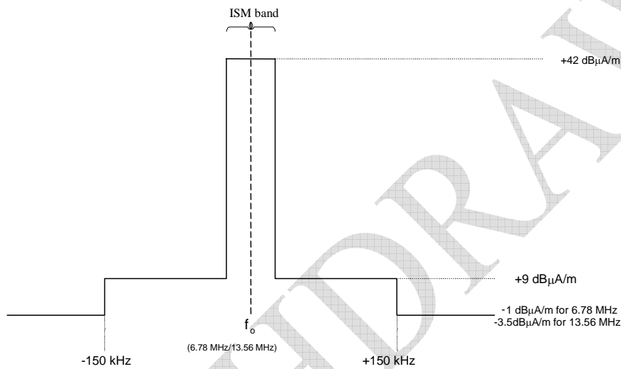
Figure 1. Magnetic field strength limits at 10 metre measurement distance
