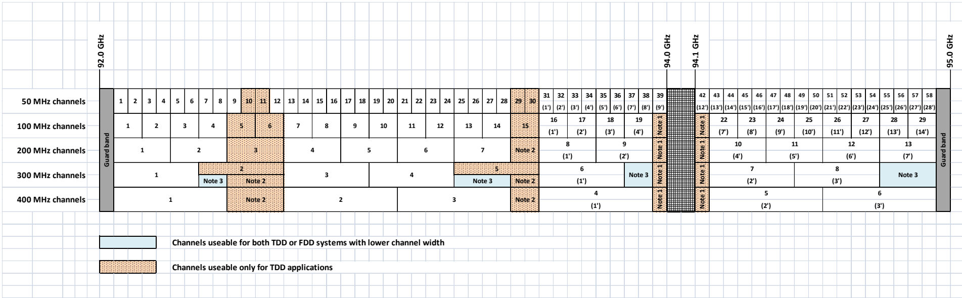
Figure 1: Channel positions for TDD and FDD applications
