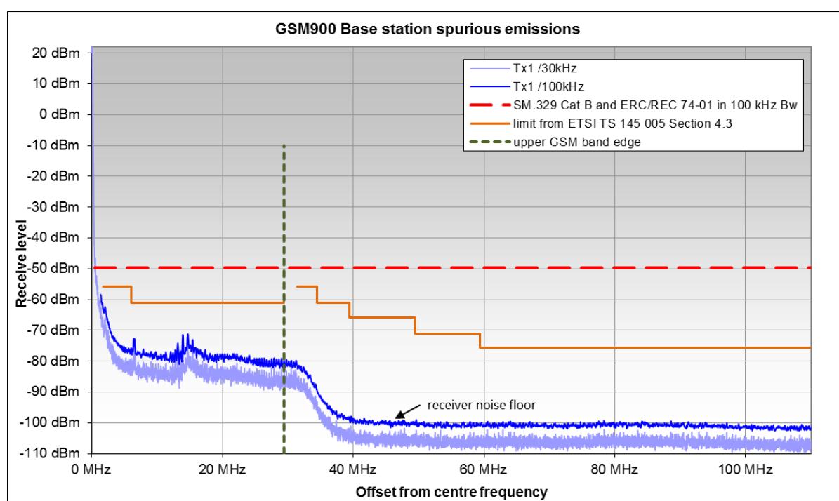
Figure 13: GSM900 spurious emissions (upper frequency range)
