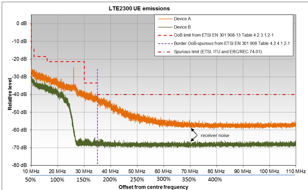
Figure 11: Unwanted emission measurements of 2 LTE 2.3 GHz UEs (RMS power, resolution bandwidth = 10 kHz)
