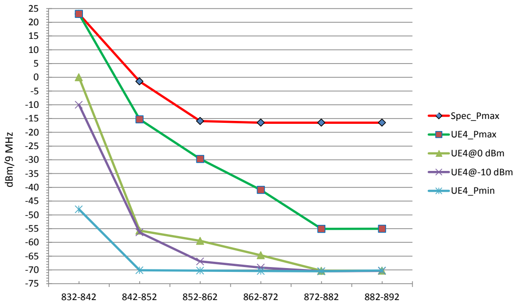
Figure 38: Measured UE#4 OOB Emissions (QPSK modulation, 50 RBs)
