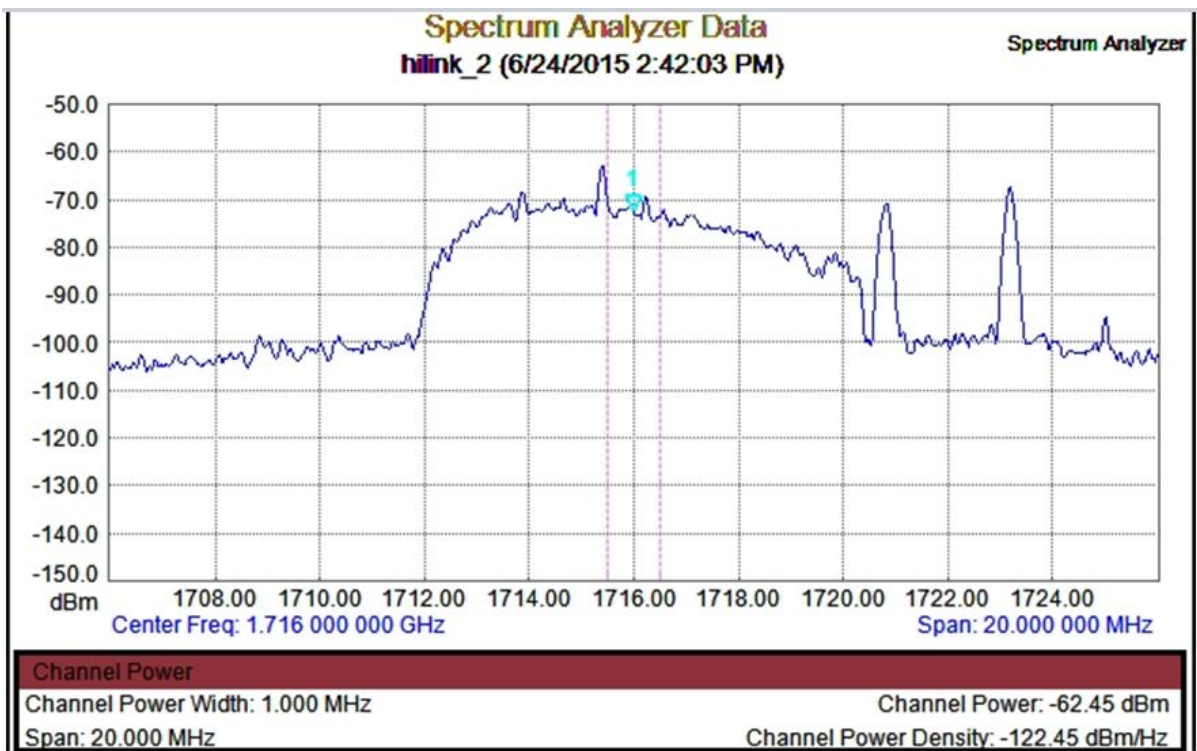
Figure 10: Emission from an LTE800 UE at the second harmonic frequency
