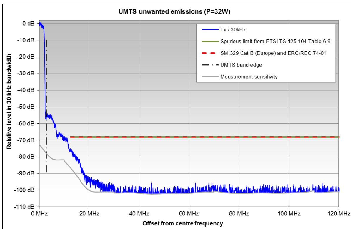
Figure 17: Spurious emissions from a UMTS base station
