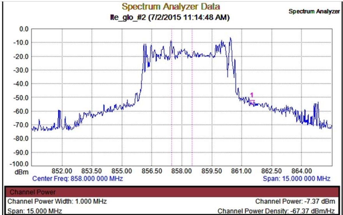
Figure 9: In-band emission from an LTE800 UE
