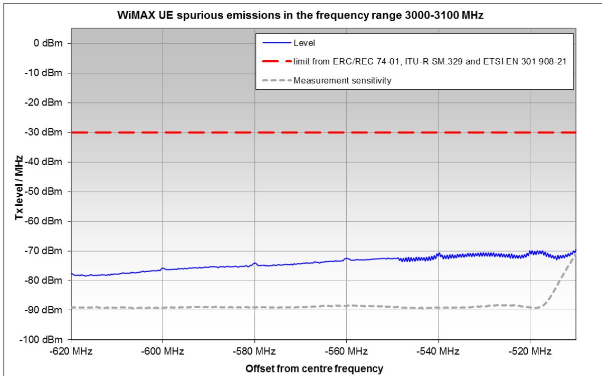
Figure 20: UE 3.6 GHz WiMAX - Emissions in radar frequency band
