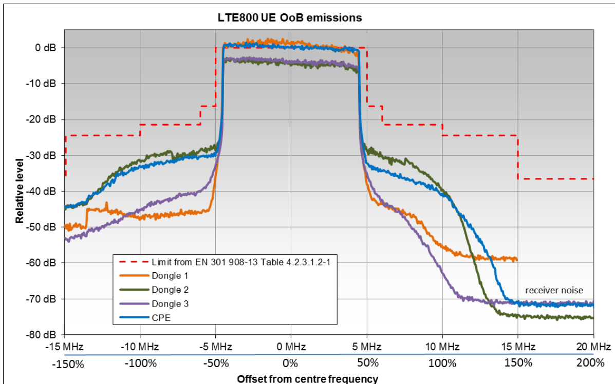
Figure 7: OoB measurements of four LTE800 UEs
