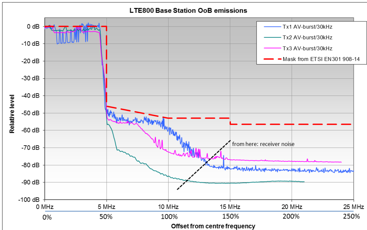
Figure 5: OoB emissions from LTE800 base stations
