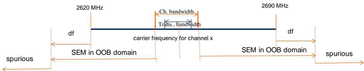
Figure 1: Out-of-band and spurious domain for E-UTRA band 7 ( df = 10\text{MHz} )
