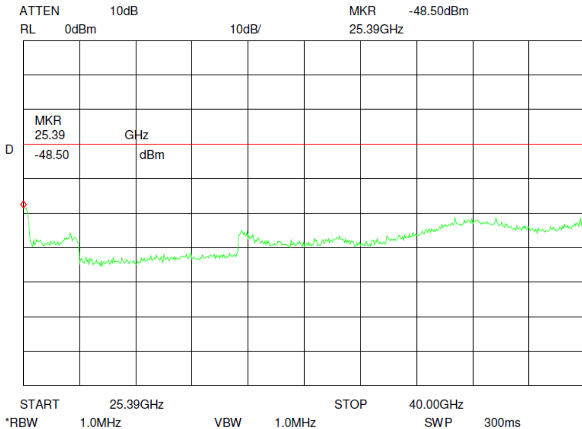
Figure 22: 25 GHz Point to Point link spurious emissions
