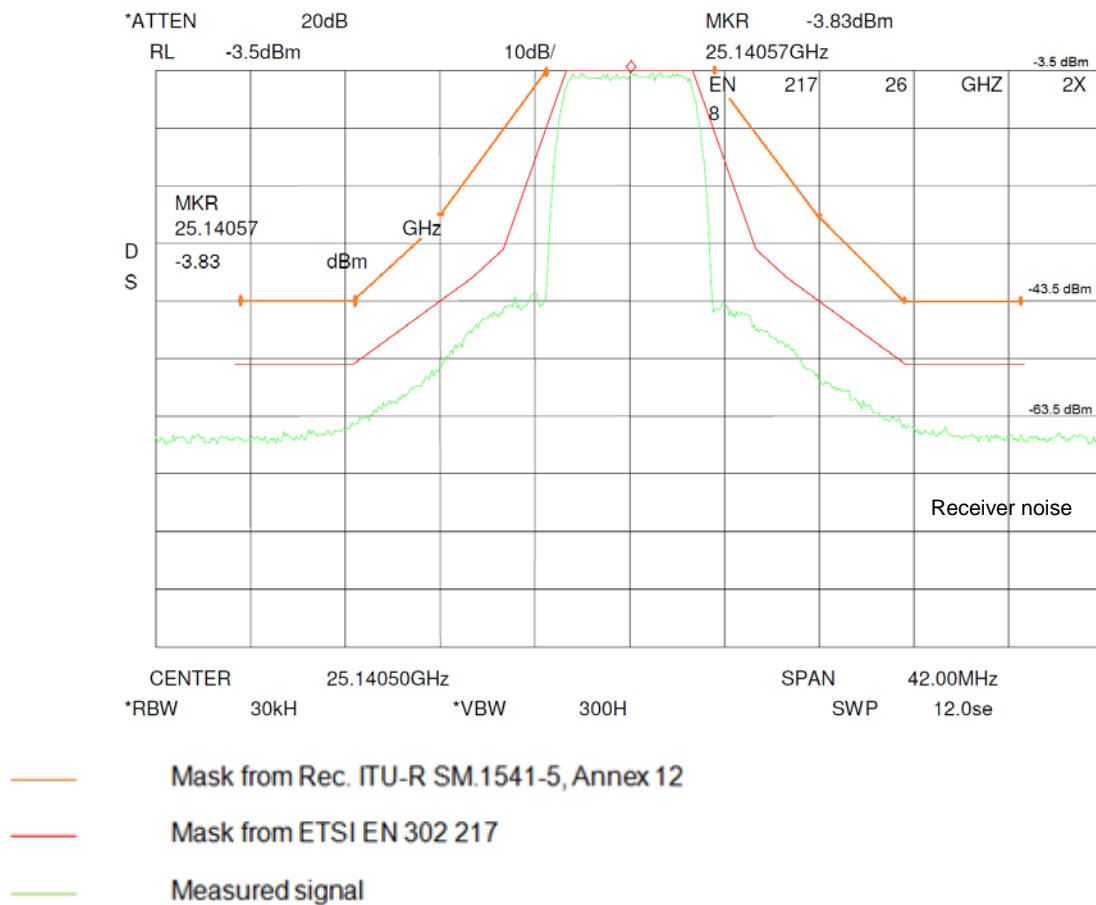
Figure 44: 25 GHz Point to Point link unwanted emissions - Device B
