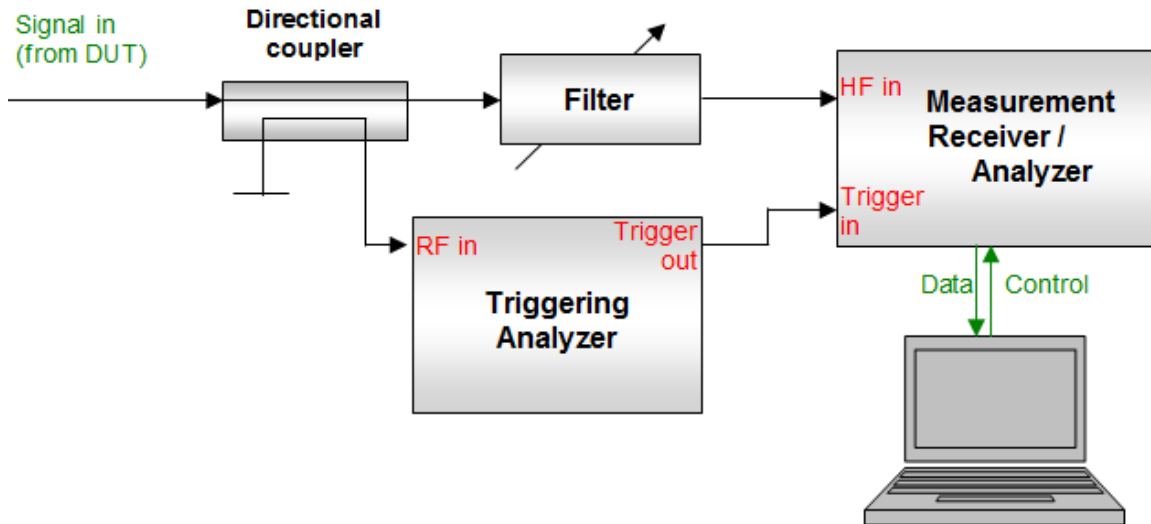
Figure 30: Setup Type 3 for measurements of TDMA systems
