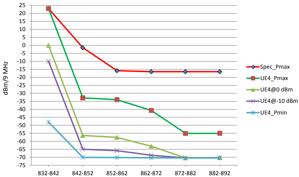
Figure 39: Measured UE#4 OoB Emissions (QPSK modulation, 12 RBs)
