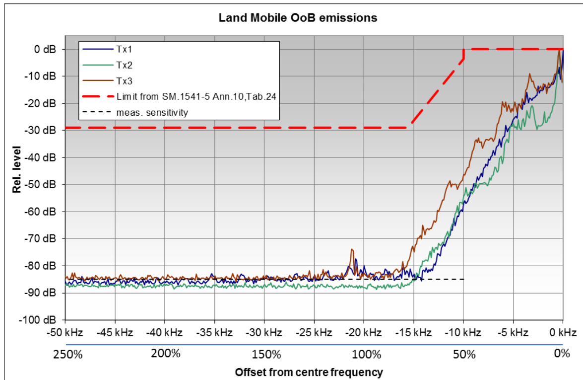
Figure 50: OoB emissions from Land Mobile stations
