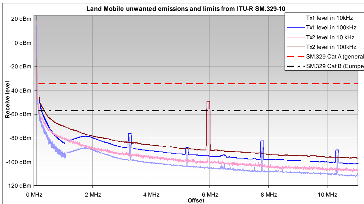
Figure 27: Land Mobile spurious emissions from two different PMR transmitters (upper frequency range)
