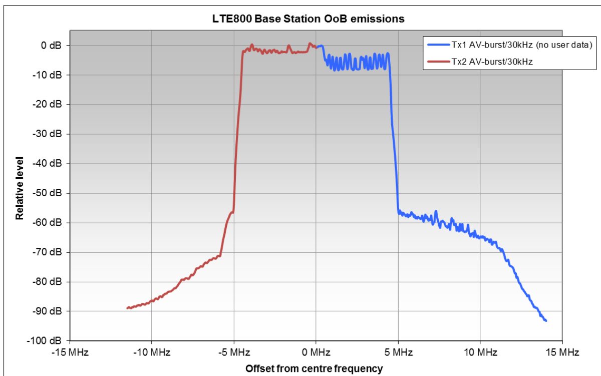
Figure 24: 'Asymmetrical' OoB spectra from an LTE800 Base Station
