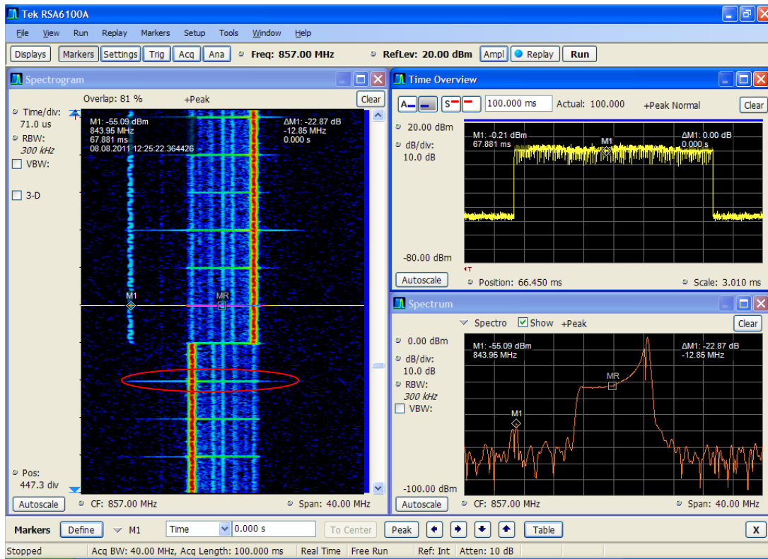
Figure 26: Spectrum, power versus time and momentary spectrum at the time marked with a line (with points M1 and MR) in the spectrogram of a randomly selected LTE800 UE, high time resolution
