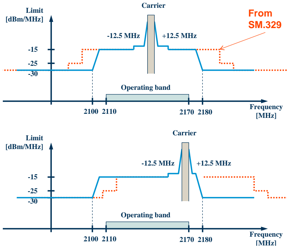
Figure 32: UTRA Category B spurious emission limits for a single 5 MHz carrier in two example carrier positions. The dotted red line shows the relevant limits from ERC/REC 74-01 [2] and Rec. ITU-R SM.329 [3]
