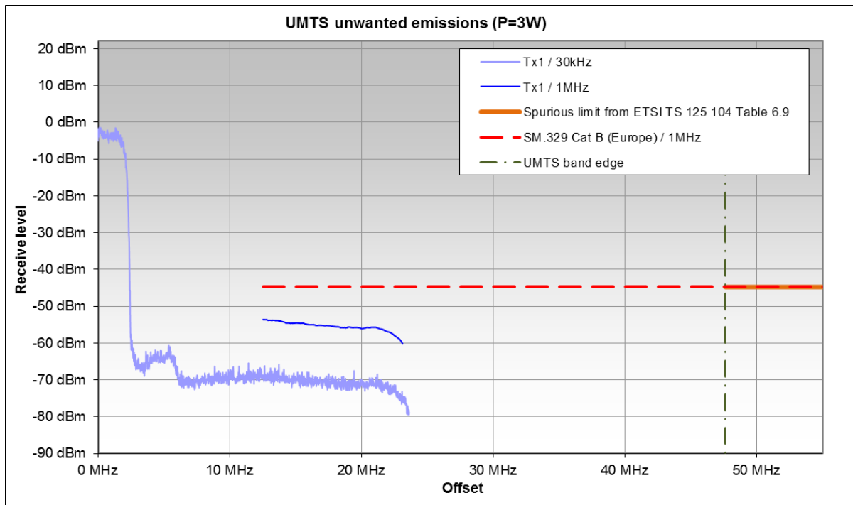
Figure 42: UMTS spurious emissions (upper frequency range)
