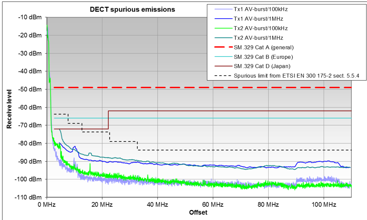
Figure 15: DECT spurious emissions (upper frequency range)
