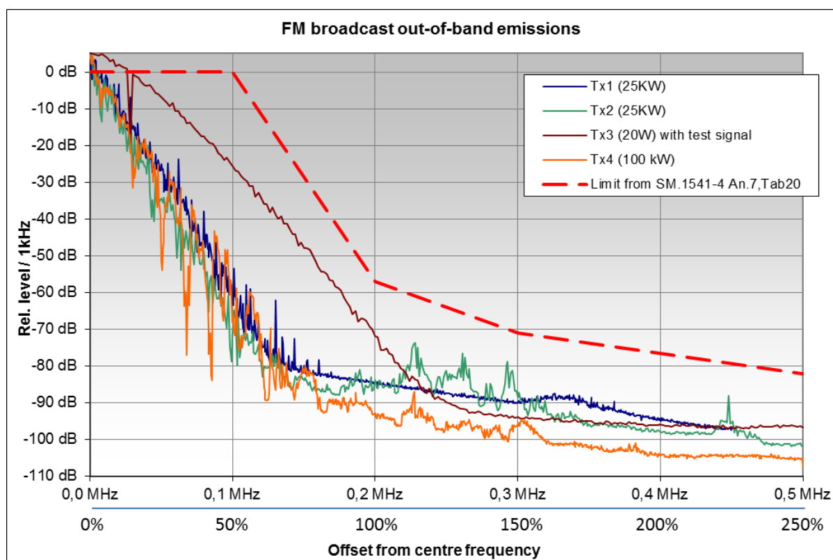
Figure 46: OoB measurements from four different FM broadcast transmitters
