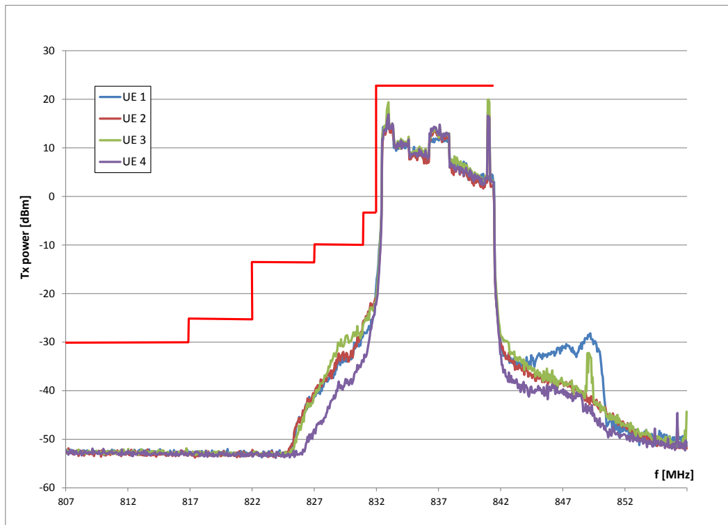
Figure 40: Comparison of LTE UE emissions (807-857 MHz, Bandwidth = 1 MHz) vs. LTE spectrum emission mask (ETSI, 2013)
