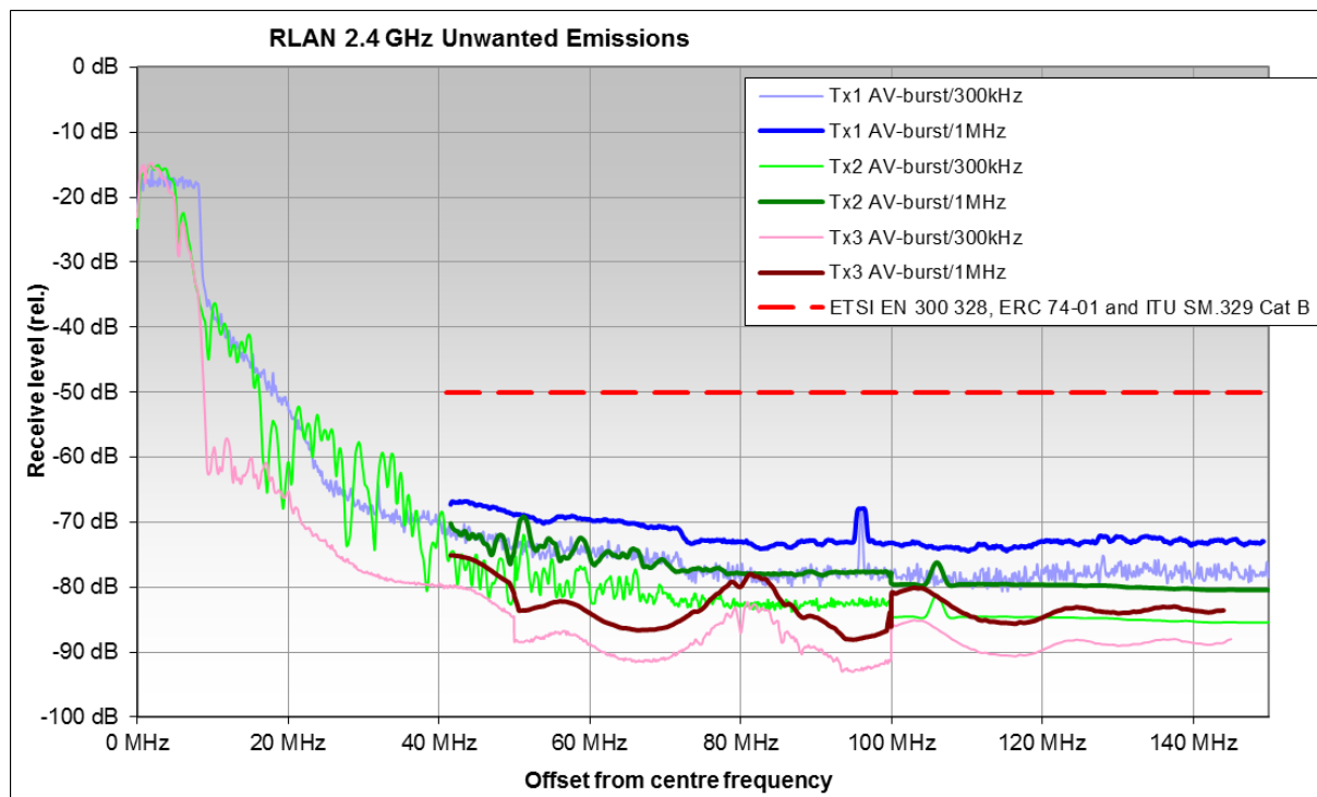
Figure 19: RLAN spurious emissions
