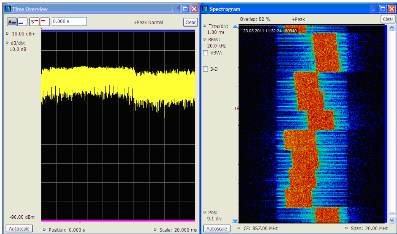
Figure 35: Power versus time and spectrogram for signal UE2
