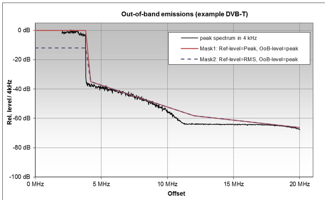
Figure 31: Different mask definitions - an example (DVB-T OoB emissions)
