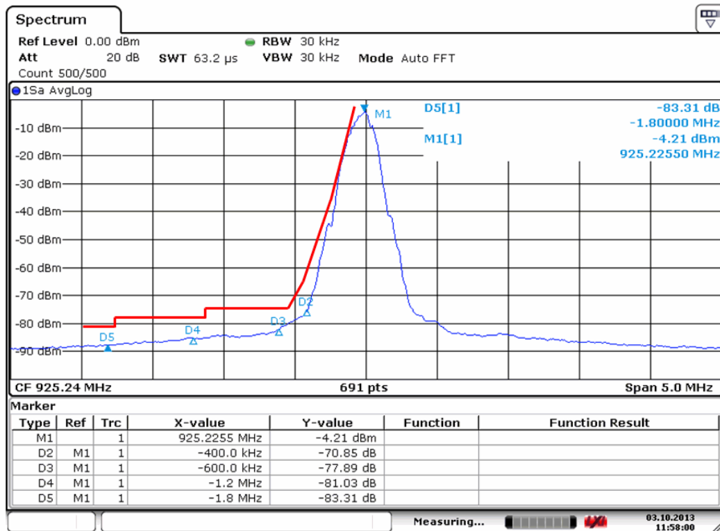
Figure 12: Measurement result of GSM900 base station test
