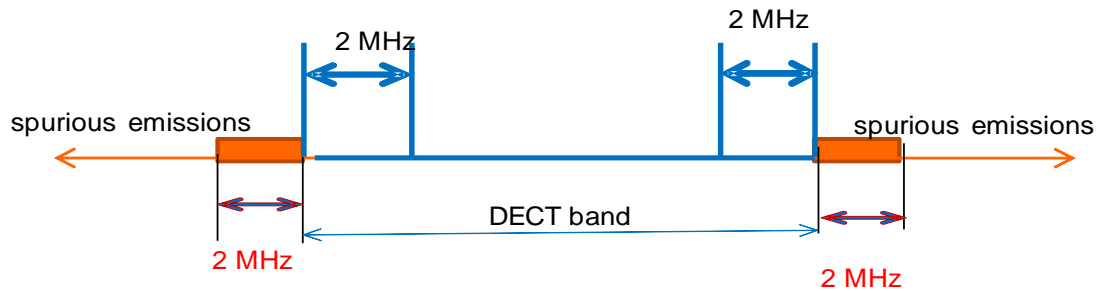
Figure 34: Clarification on DECT OoB and spurious emissions terminology
