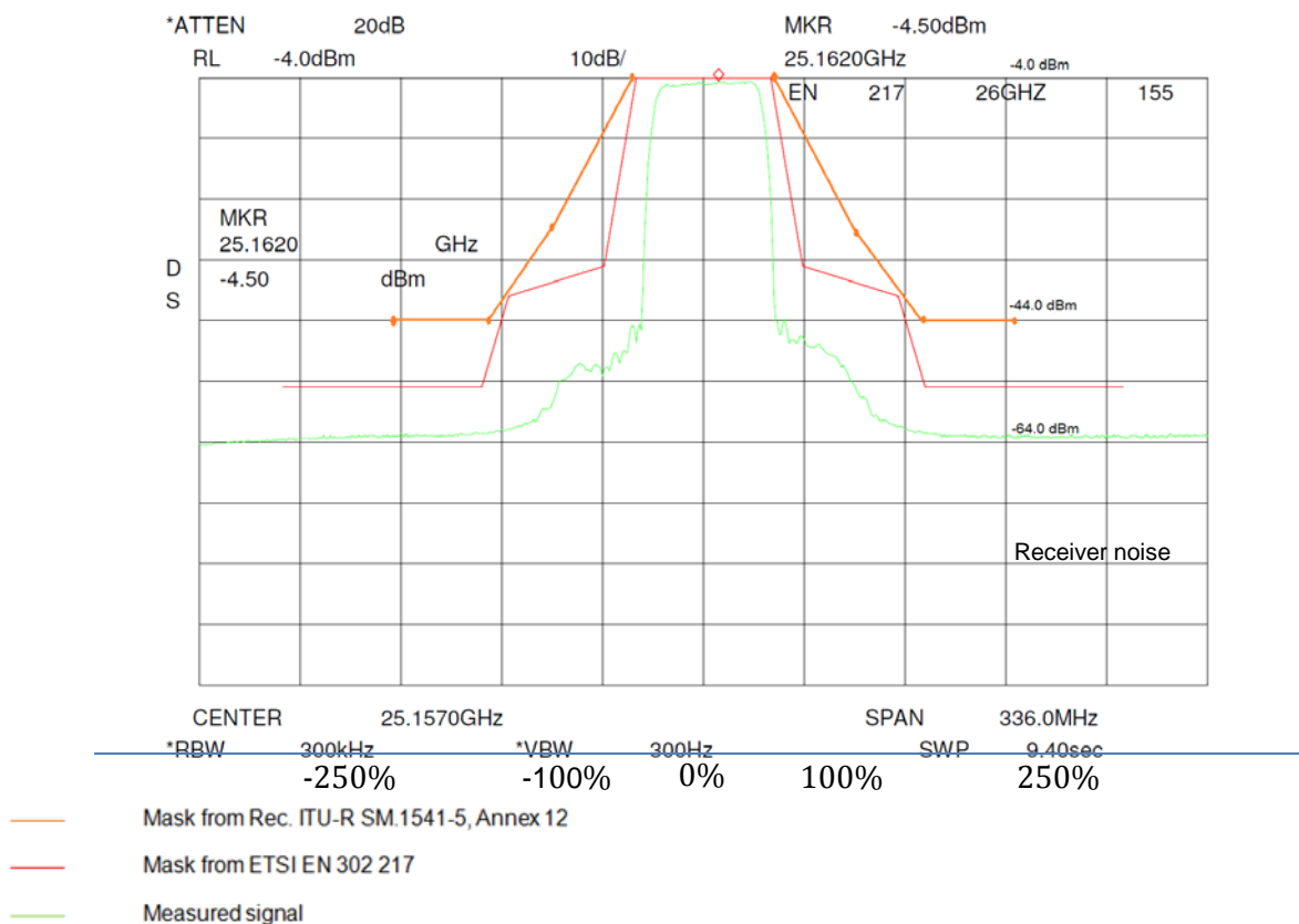
Figure 21: 25 GHz Point-to-Point link unwanted emissions
