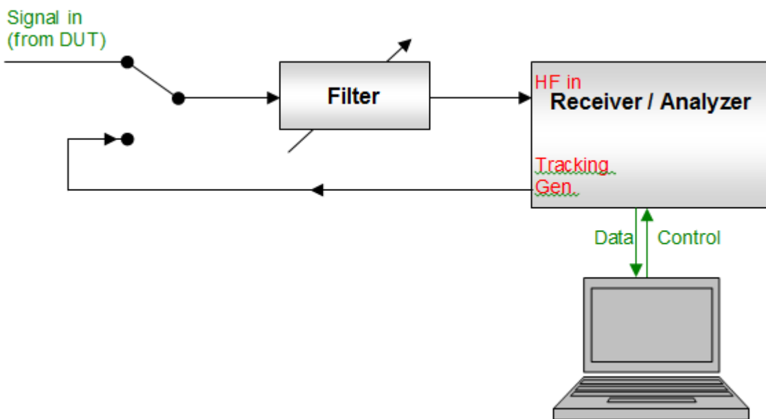
Figure 29: Principle measurement setup Type 2
