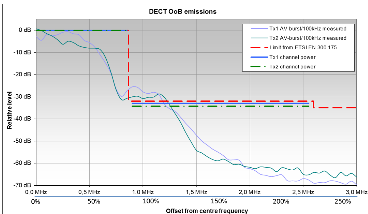
Figure 14: DECT OoB emissions (upper frequency range)
