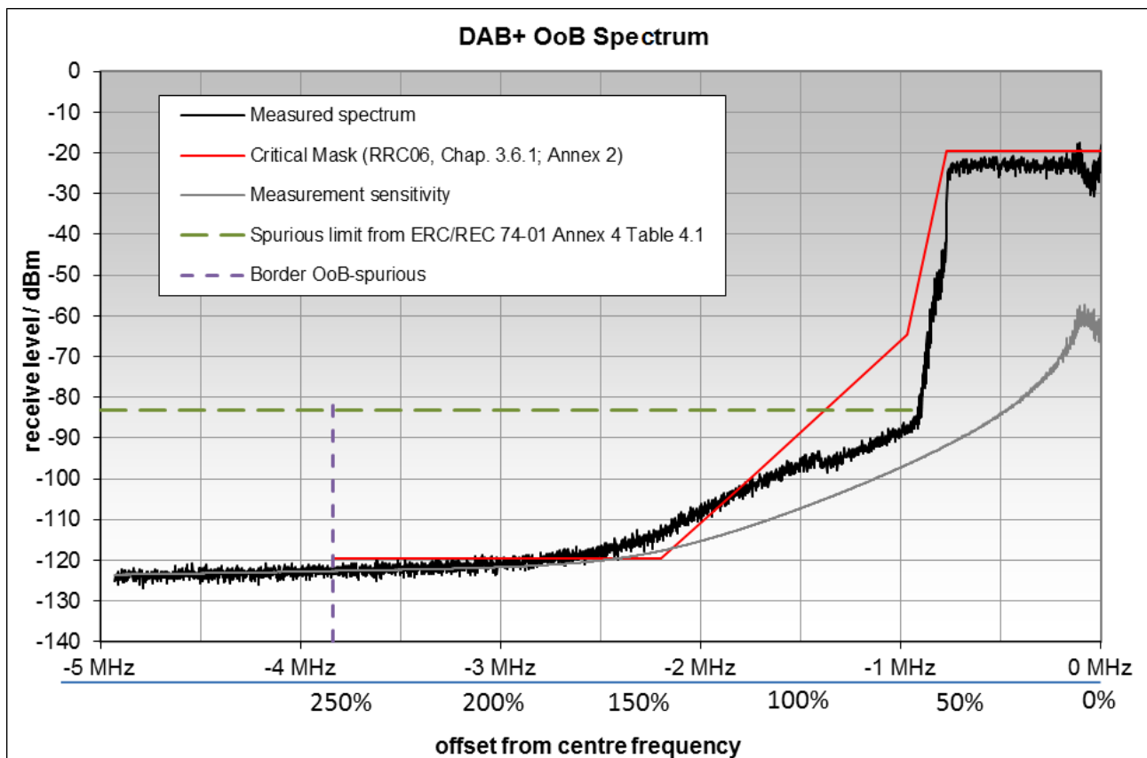
Figure 2: OoB measurements from a DAB+ transmitter
