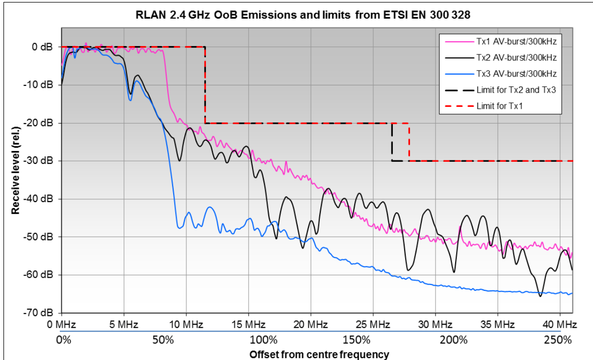
Figure 18: RLAN OoB emissions
