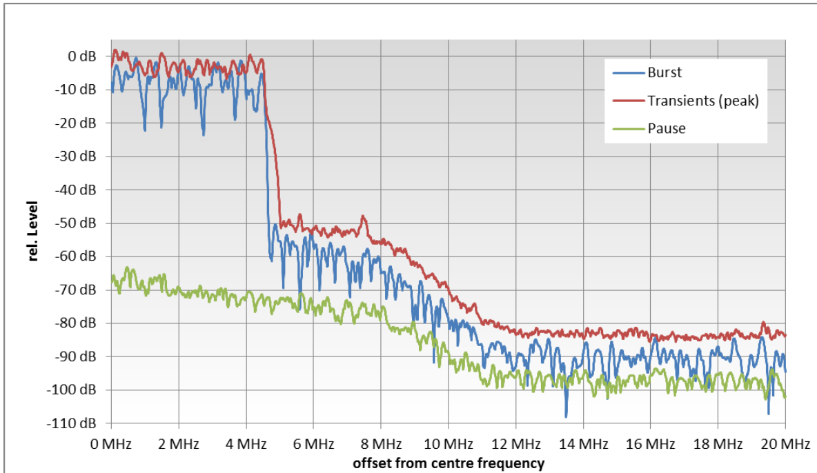
Figure 25: LTE800 BS: OoB emissions at different times
