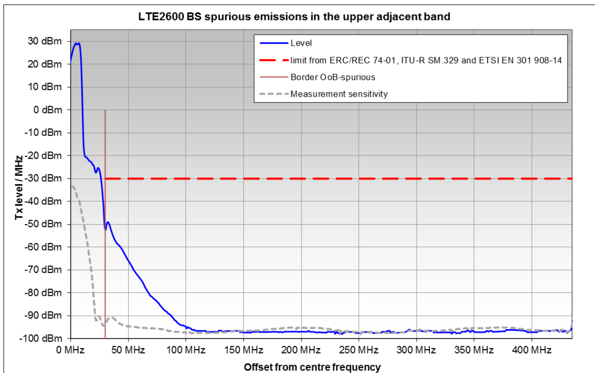
Figure 41: LTE2600 BS spurious emissions (Bandwidth = 1 MHz)
