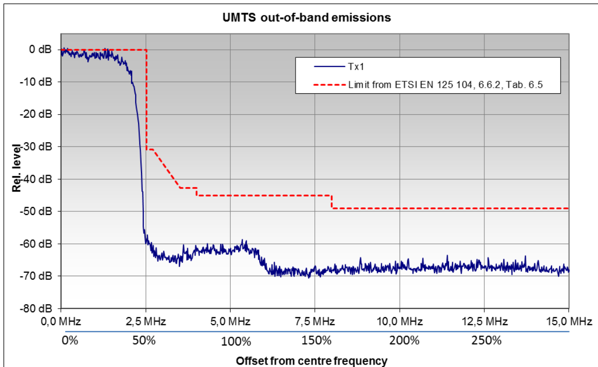
Figure 16: OoB emissions from a UMTS base station
