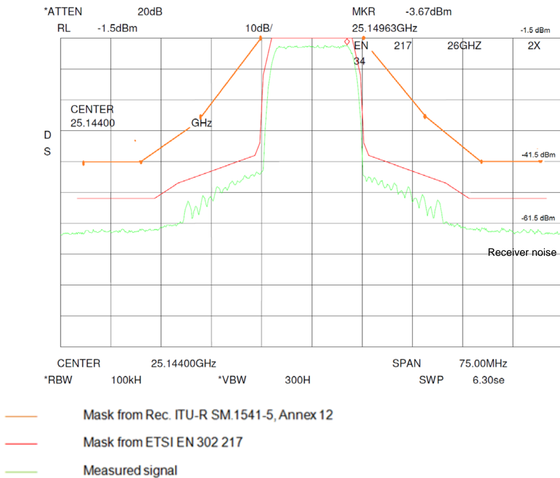
Figure 45: 25 GHz Point to Point link unwanted emissions - Device D
