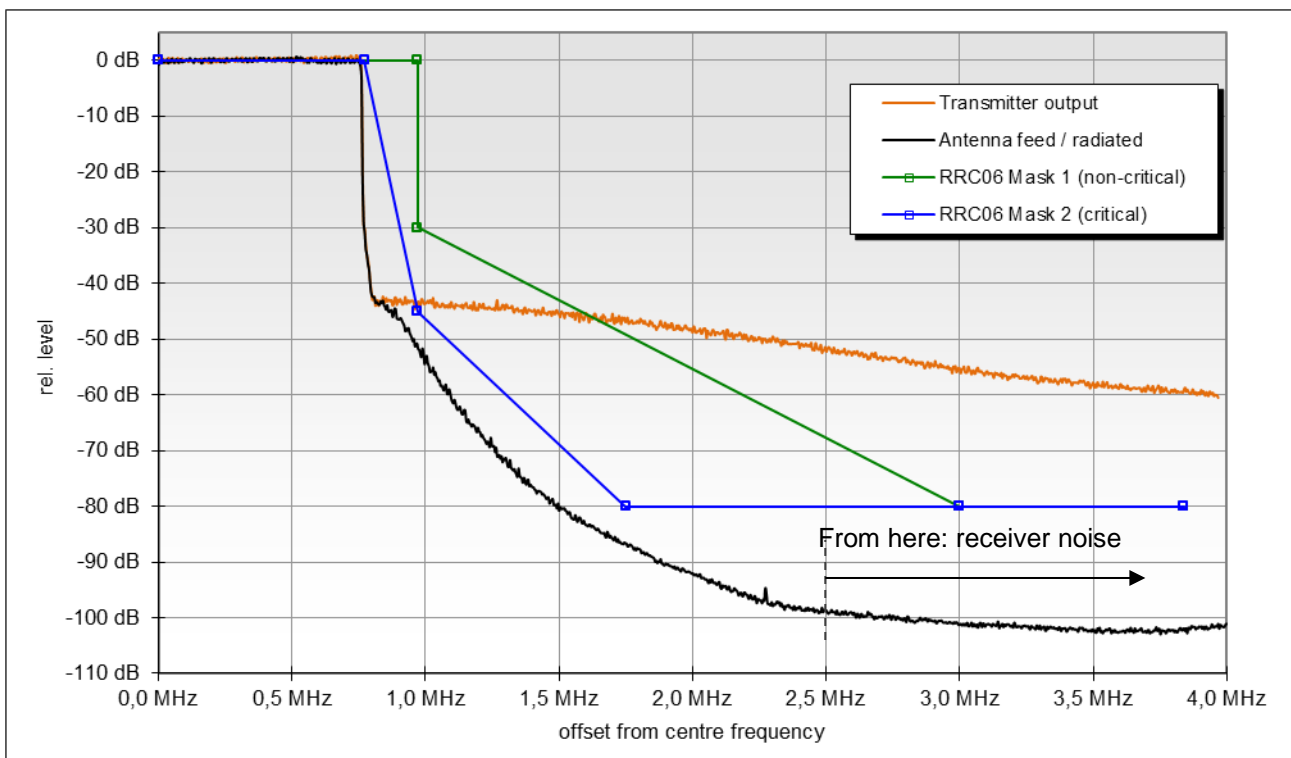
Figure 23: DAB unwanted emissions in the OoB domain
