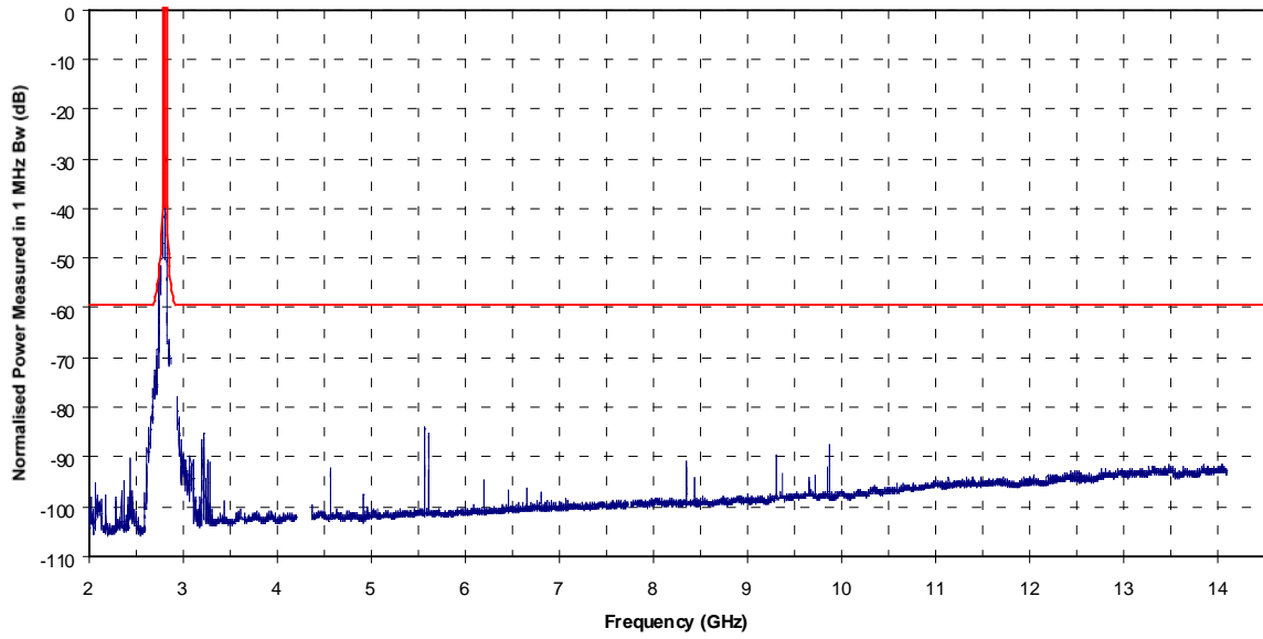
Figure 51: Civil Air traffic Control radar #1
