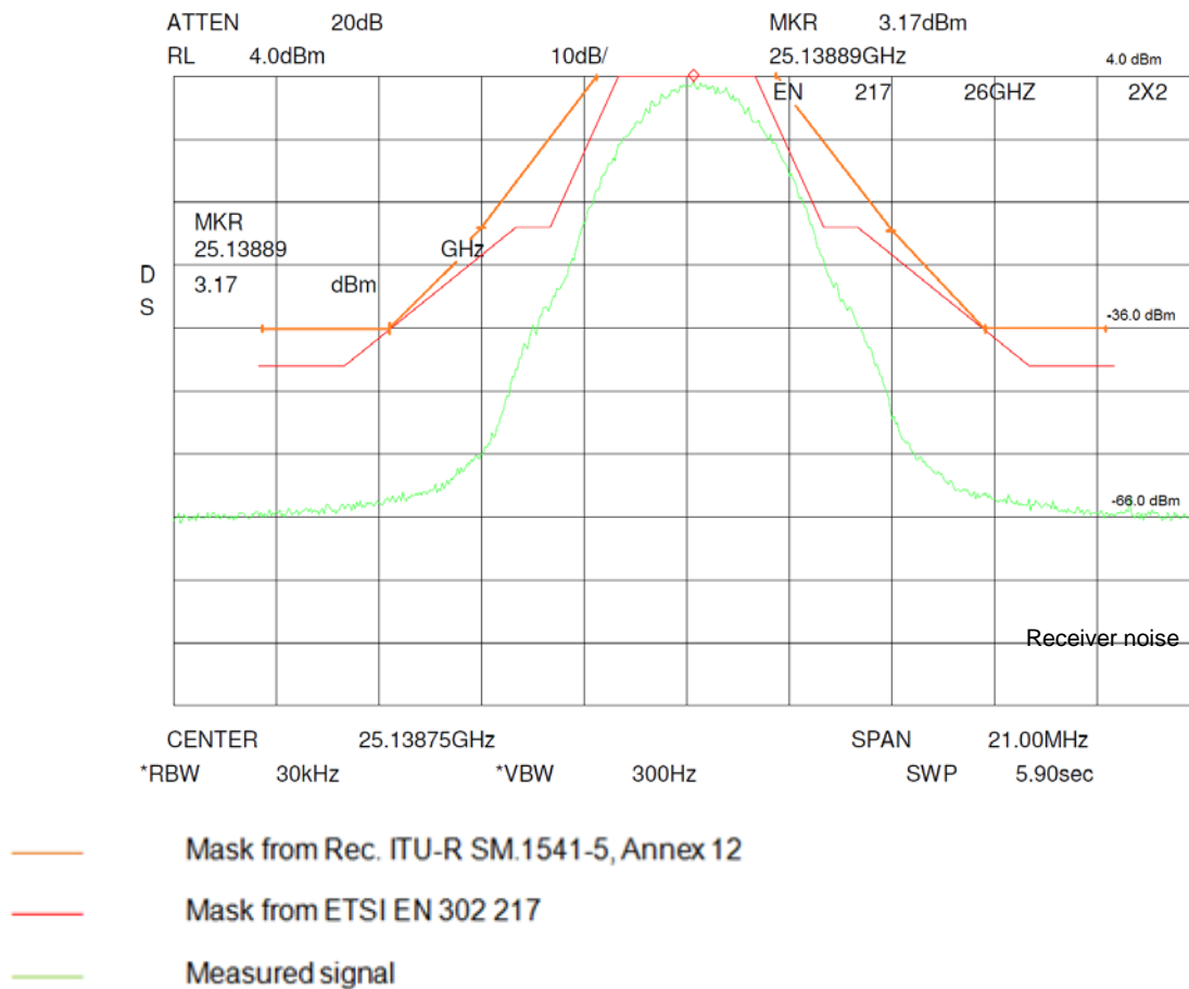
Figure 43: 25 GHz Point to Point link unwanted emissions - Device A
