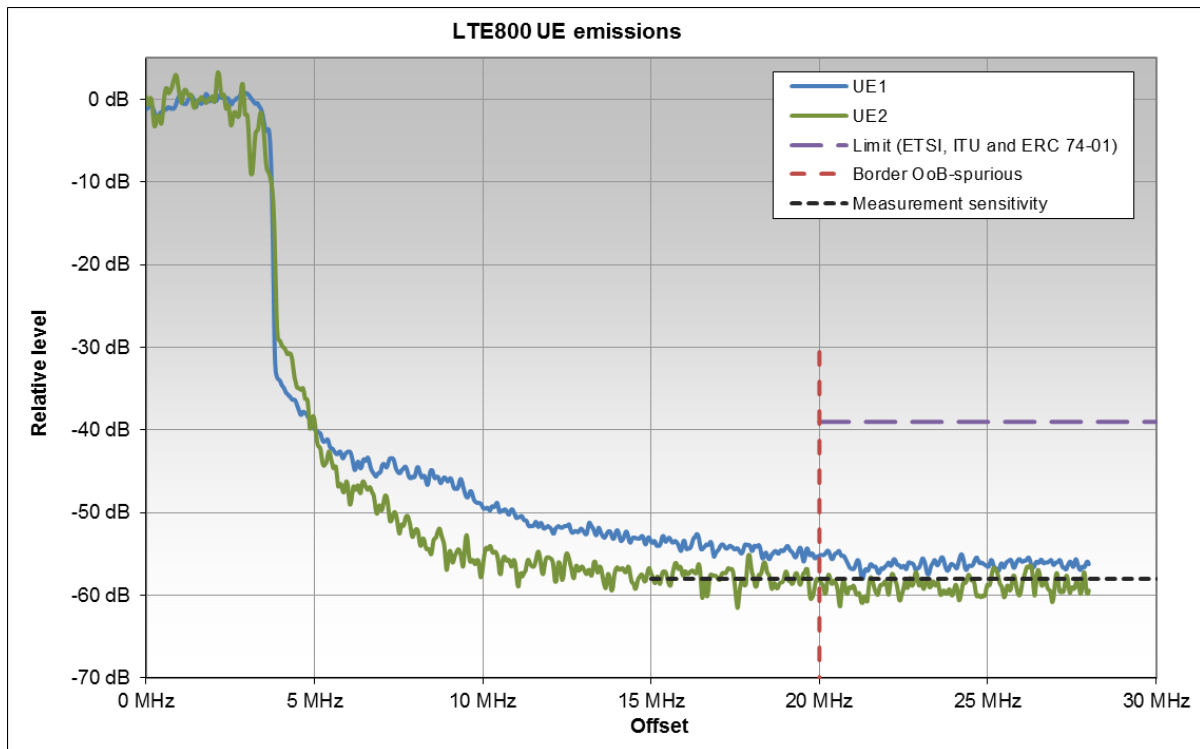
Figure 8: Emissions from two LTE800 UEs
