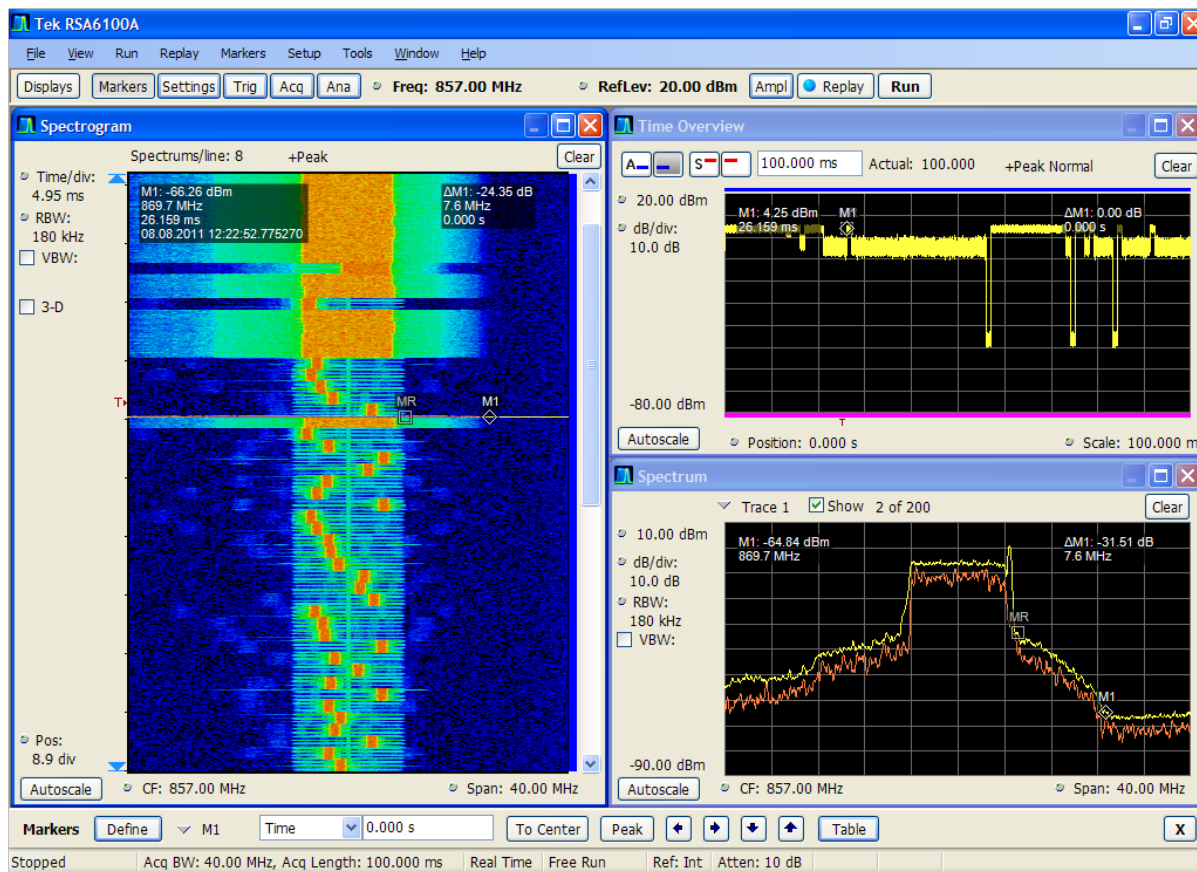
Figure 37: Example of Out-of-Band emissions of a randomly selected LTE terminal. Spectrogram (left), power vs. time (upper right) and spectrum (yellow: whole acquisition time; orange: time instant marked with a line in the spectrogram)
